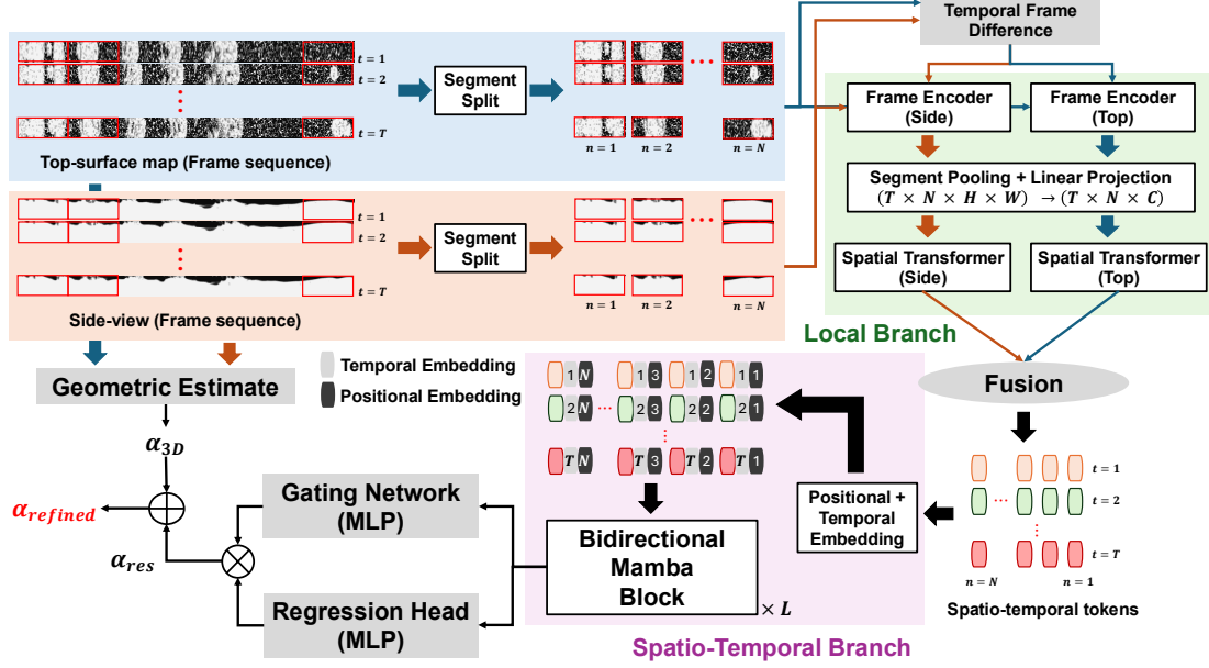
Figure 2. Overview of VFNet network architecture. Top phase maps and side views are divided into N segments and encoded into d -dimensional tokens by the Local Branch , which are then fused and arranged into spatio-temporal tokens. The Spatio-Temporal Branch applies L stacked Bidirectional Mamba blocks to capture inter-frame and inter-segment dependencies. A gated Regression Head predicts a residual correction \alpha_{\text{res}} that refines the geometric prior \alpha_{3D} , yielding the final estimate, \alpha_{\text{refined}} .
