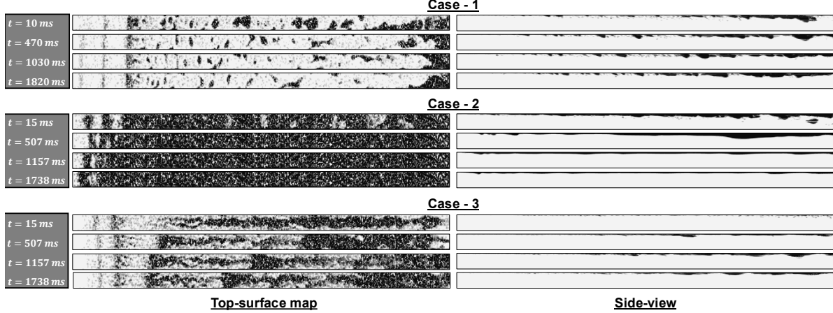
Figure 4. Sample synchronized dual-view sequences from our CFD dataset, shown for three distinct simulation cases. For each case, we display the representative top-surface reflection-based phase map (left) and the corresponding side-view shadowgraph (right) at four representative time steps. The two perpendicular views capture complementary information about the vapor distribution, and the cases exhibit a wide range of bubble dynamics and flow morphologies, from dispersed bubbly structures to elongated coalesced vapor structures.
