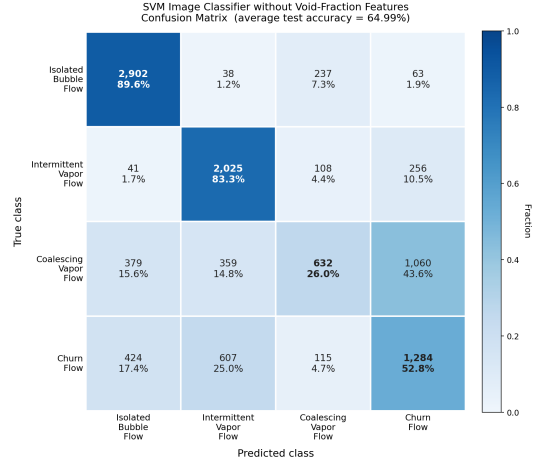
(b) SVM — w/o vf features
