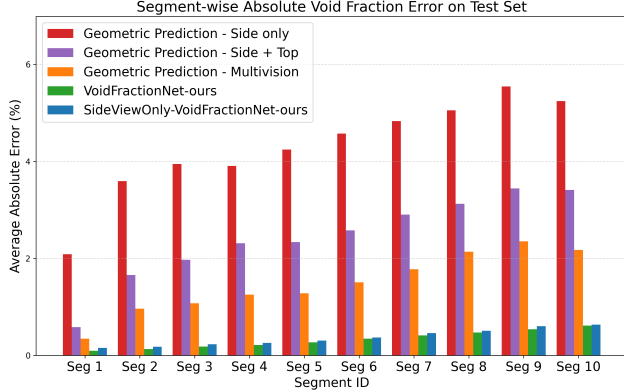
(a) VFNet vs. geometric baselines.
