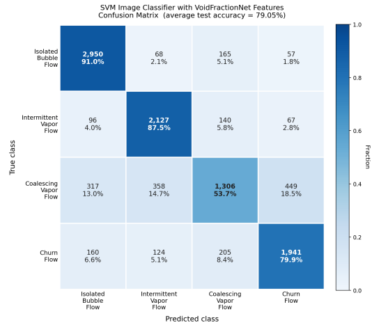
(f) SVM — VFNet features
