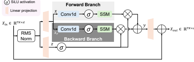
Figure 3. Bidirectional Mamba block from Zhu et al. [59]. After RMSNorm and linear projection, the forward branch processes the token sequence x and the backward branch its reverse x_r , each through a Conv1d, SiLU activation ( \sigma ), and selective SSM block. The branches are gated by a SiLU-activated projection z , summed, and combined with a residual connection to yield X_{out} .
