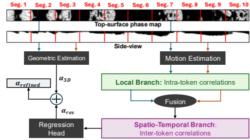
Figure 1. Overview of our proposed VFNet. From the side view shadowgraph and top-surface phase map, a fast geometric estimator produces an initial void fraction \alpha_{3D} . VFNet predicts a learned residual that is added to this prior, yielding a refined per-segment estimate.
