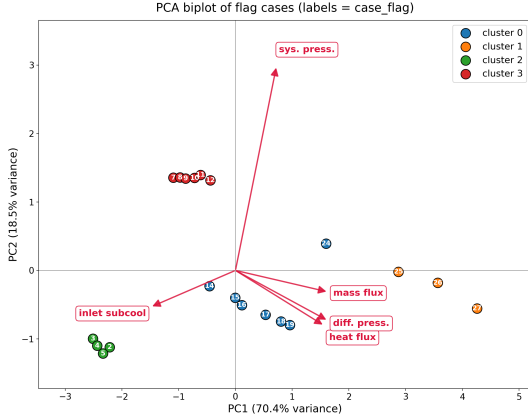
Figure 7. PCA projection of the 20 experimental cases based on their physical parameters. The K-Means clustering separates the cases into four flow-pattern classes, with each cluster corresponding to a distinct flow regime.
