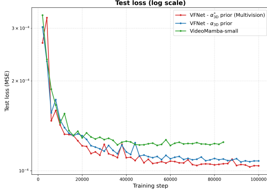
(a) Test loss (MSE, log scale) against training step. Both runs of VFNet clearly separate from VideoMamba-small and settle 15–18% lower. Between the two priors, \alpha_{3D}^* converges slightly faster and ends 3.9% lower.
