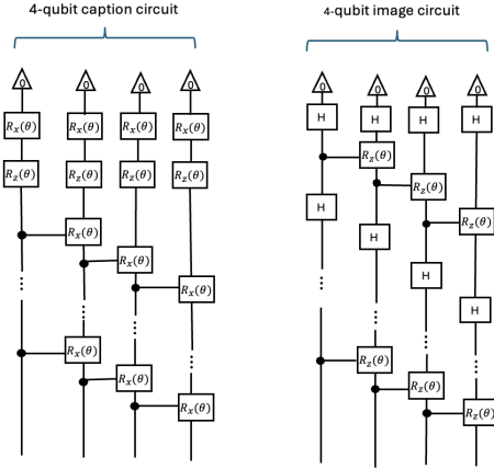
Fig. 2: Four-qubit quantum circuits used in Stage 1 for single-object image–caption alignment. The caption circuit (left) is constructed using the Sim4 ansatz with trainable parameterized rotations, while the image circuit (right) uses the IQP ansatz to angle-encode PCA-reduced CLIP image features. Both circuits produce 4-qubit pure states, whose fidelity defines the image–caption similarity during training and is subsequently estimated using the destructive SWAP test.
