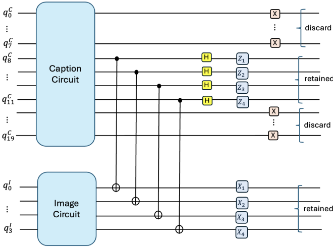
Fig. 4: Hardware implementation of the destructive SWAP test. The retained output qubits of the caption circuit are compared with the corresponding output qubits of the image circuit using Bell-basis measurements. The measured outcomes are combined to estimate the Hilbert–Schmidt overlap \text{Tr}(\rho_C \rho_I) , which equals the Uhlmann fidelity for a pure image state. The figure depicts the Stage 2 hardware configuration; Stage 1 follows the same procedure using two 4-qubit circuits.
