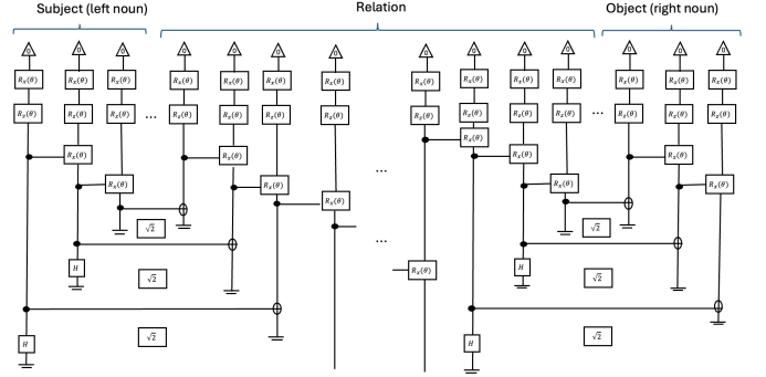
Fig. 3: Variational Quantum Circuit for the relational caption obtained by applying the Sim4 ansatz to the corresponding DisCoCat diagram. The retained s -type output qubits represent the sentence meaning, while the remaining qubits are discarded to obtain the reduced caption density matrix \rho_C .
