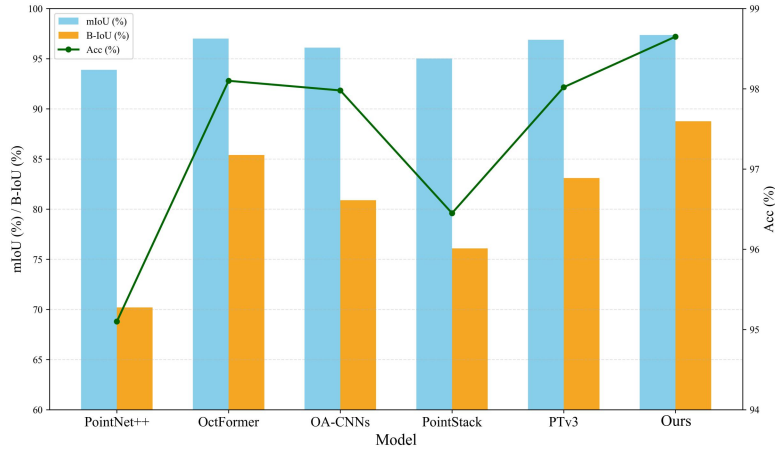
Figure 8. Comparative performance of different point cloud segmentation models. Acc, accuracy; mIoU, mean Intersection over Union; B-IoU, boundary Intersection over Union. Higher values indicate better segmentation performance.
