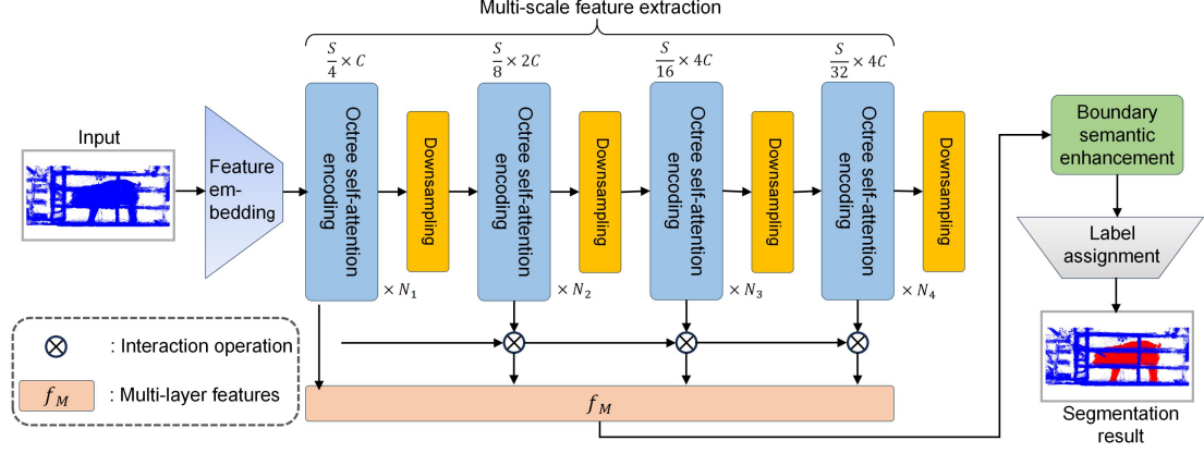
Figure 4. Overall architecture of the proposed boundary-aware pig point cloud segmentation network. The network uses Octree Transformer as the backbone and integrates multi-scale feature fusion, soft-distance boundary supervision, and bidirectional semantic-boundary feature interaction for pig point cloud segmentation.
