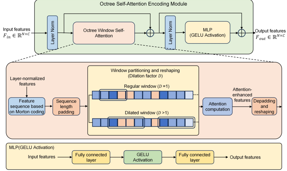
Figure 5. Architecture of the octree self-attention encoding module. Non-empty octree nodes are encoded using Morton ordering and processed through local and dilated window self-attention to capture both local geometric details and broader contextual information.
