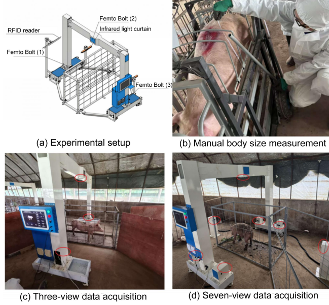
Figure 1. Data acquisition system and field setup for pig point cloud collection. The system integrates multi-view depth cameras, infrared triggering, directional guide fences, and RFID-based individual identification for synchronized point cloud acquisition in a commercial pig housing environment.
