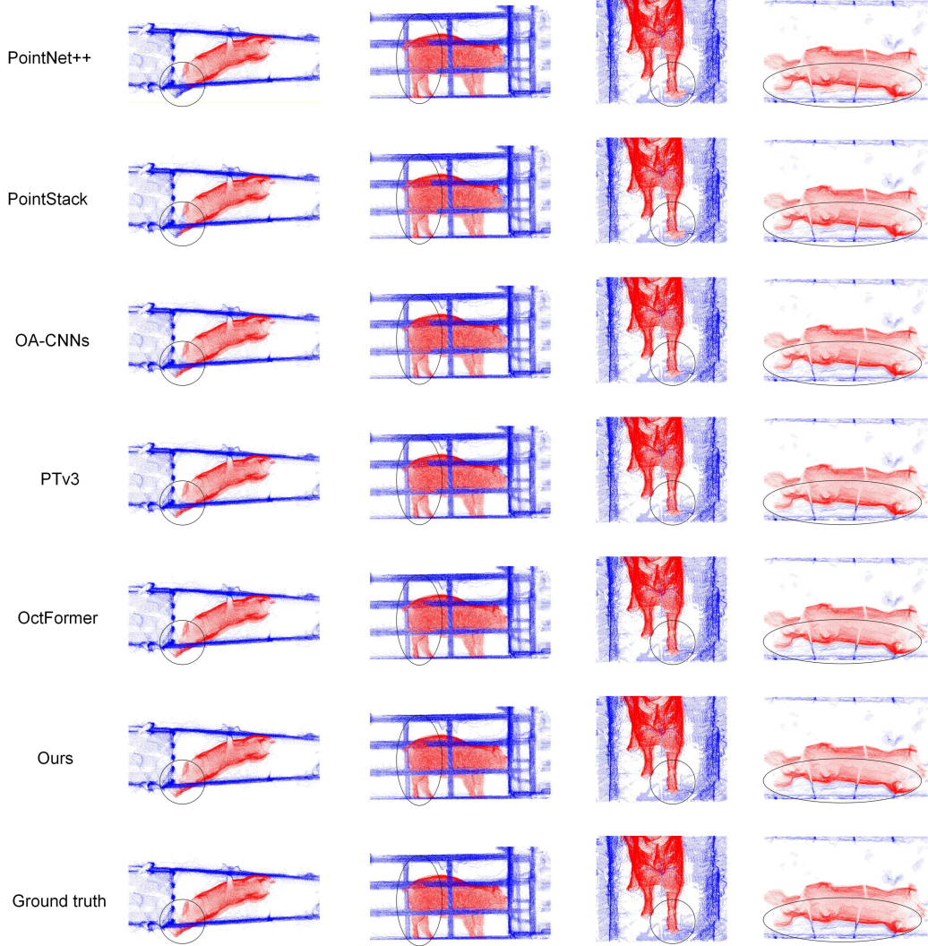
Figure 9. Qualitative comparison of segmentation results obtained by different point cloud segmentation models. The comparison illustrates segmentation differences in boundary-contact regions between the pig body and background structures, including railings, fences, and the floor.
