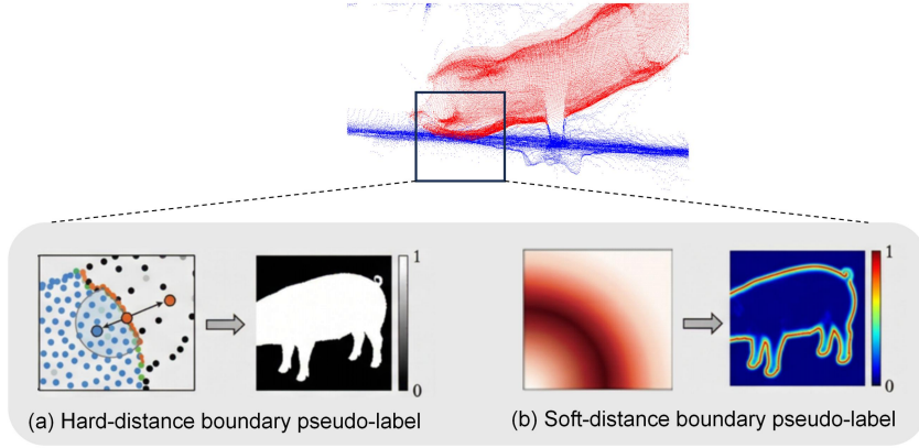
Figure 6. Illustration of the soft-distance boundary pseudo-labeling strategy. Boundary supervision is generated according to the distance from each point to its nearest out-of-class point, producing a continuous boundary probability that decays from the contact boundary to non-boundary regions.
