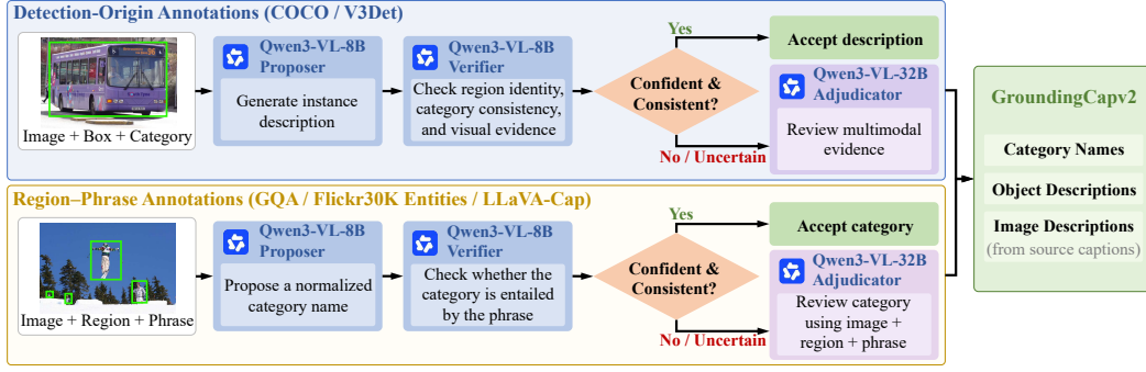
Figure 2: Confidence-routed GroundingAgent-Opt. Qwen3-VL-8B agents curate GroundingCap-1M category and object annotations, routing uncertain cases to Qwen3-VL-32B. Together with inherited image descriptions, curated annotations form GroundingCapv2’s tri-level supervision.
