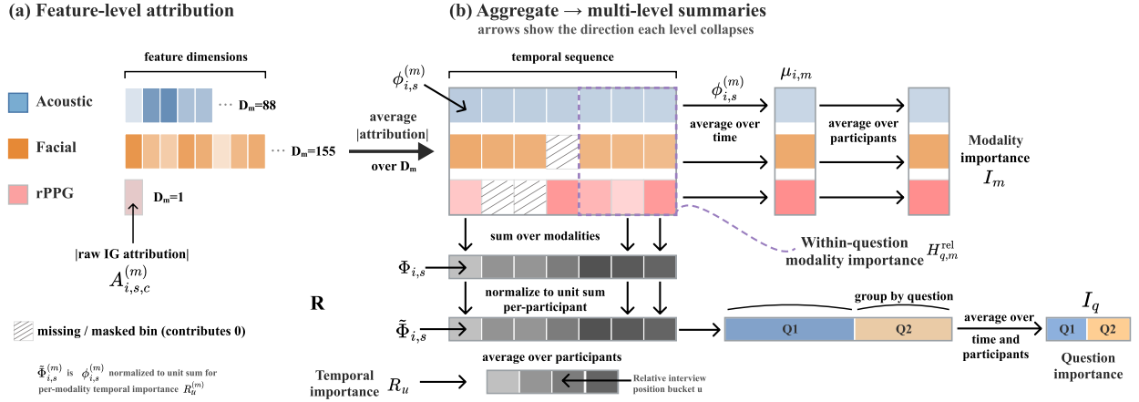
Fig. 7. (a) After training, IG assigns a scalar attribution A_{i,s,c}^{(m)} to each feature c of modality-feature m at temporal bin s for participant i . Averaging the absolute attributions over the modality-feature's D_m dimensions and gating by the availability mask (hatched bins are missing and contribute 0) reduces the attributions of all features c to one score per temporal bin \phi_{i,s}^{(m)} . (b) These per-temporal-bin scores are aggregated along the different axes, and arrows indicate the dimensions along which the attributions are aggregated to produce the modality importance I_m , question importance I_q , within-question modality importance H_{q,m}^{rel} , and temporal importance R_u .
