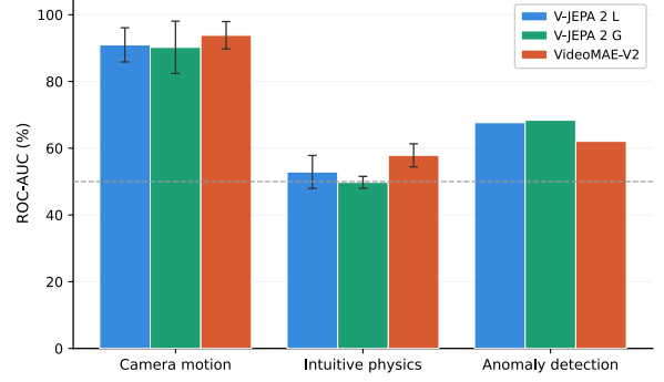
Figure 2. Mean Test ROC-AUC (%) per task family. Each group of bars corresponds to one task family (Camera Motion, Intuitive Physics, and Anomaly Detection), with individual bars showing results for V-JEPA 2 Large (blue), V-JEPA 2 Giant (green), and VideoMAE-V2 (orange). Each bar reports the mean ROC-AUC on the test set, averaged across all tasks within that family. Error bars indicate \pm 1 standard deviation across tasks within each family; Anomaly Detection has no error bars as it contains a single task. The gray dashed line marks the chance level (50%).
