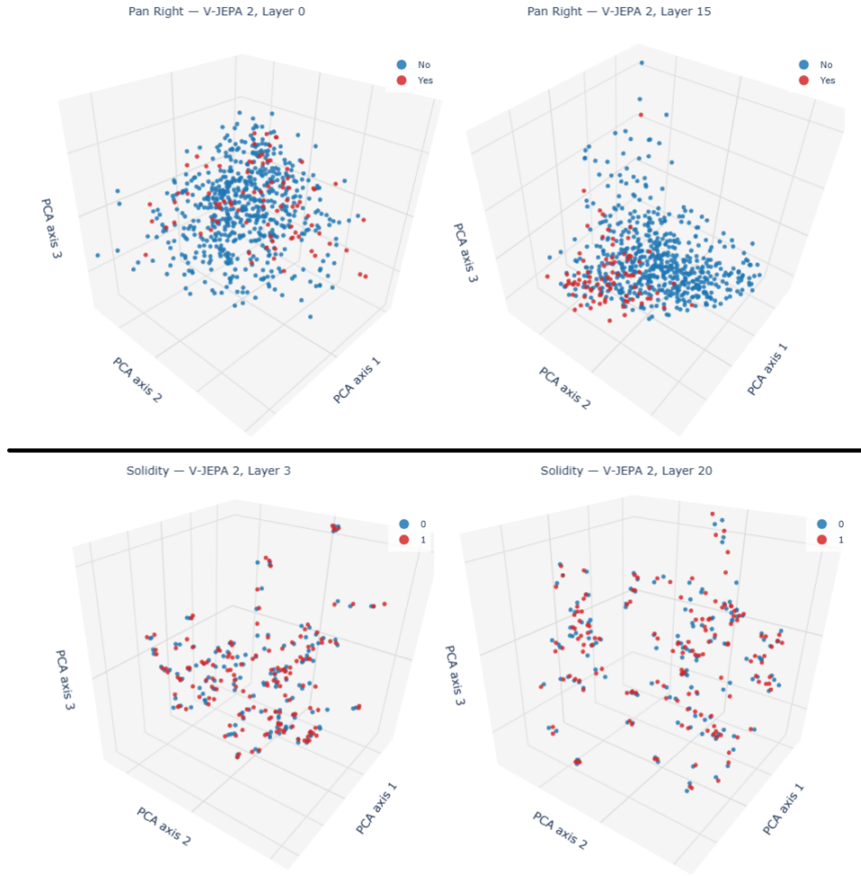
Figure 7. 3D PCA projections of frozen features coloured by class label. Top row: CameraBench (pan right task) at early layer 0 and the best-performing layer 15, showing emerging class separation at mid-depth. Bottom row: IntPhys 2 (solidity condition) at early layer 3, the apparent best layer, and a later layer 20, showing no class separation at any depth—possible and impossible events are indistinguishable in the feature space.
