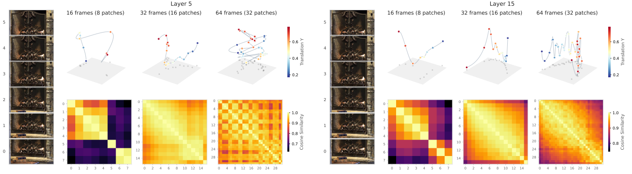
Figure 4. Temporal representation structure across frame counts and layers (V-JEPA 2L, RealEstate10K (Zhou et al., 2018)). The left and right panels show Layer 5 and Layer 15, respectively, analyzed on the same video clip with predominantly single-direction camera motion. Here, the video is translating upwards. Within each panel, columns correspond to three temporal resolutions: 16, 32, and 64 input frames (8, 16, and 32 temporal patches, respectively). The top half of each panel shows the 3D PCA projection of the temporal patch features (computed as in Eq. 1), coloured by camera translation along the y-axis. The bottom half shows the pairwise cosine-similarity matrix indexed by temporal patch position. Higher values (lighter colours) indicate more similar representations.
