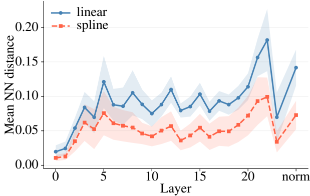
Figure 6. Nearest-neighbour (NN) distance steering results. For each interpolated latent representation, we compute the Euclidean distance to the closest temporal feature from the original video clip. Lower values indicate that the steered trajectory remains closer to the empirical representation manifold. Across nearly all evaluated layers, spline steering consistently achieves lower mean NN distances than the linear path. Shaded regions denote \pm 1 standard deviation over 200 evaluation clips.
