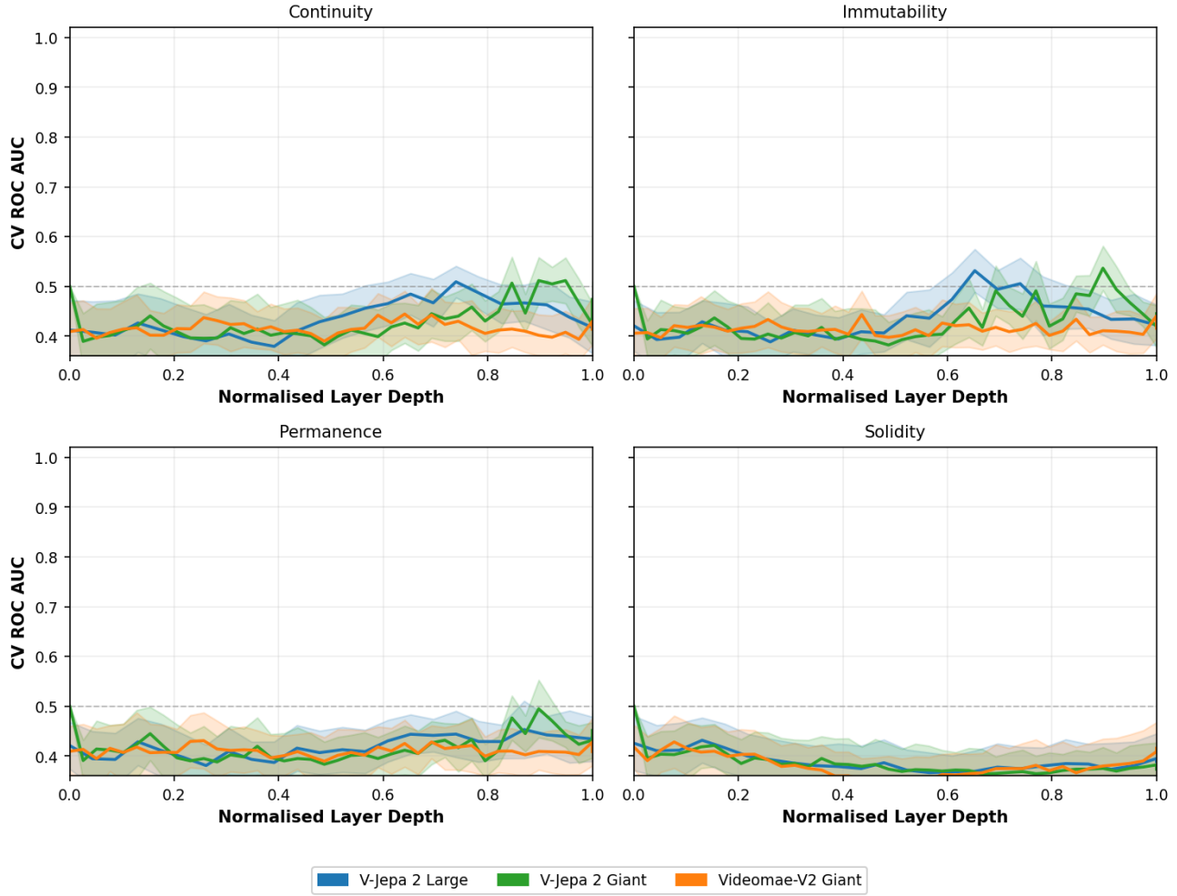
Figure 9. Layerwise cross-validation ROC AUC for individual intuitive physics subtasks (IntPhys 2 dataset): continuity, immutability, permanence, and solidity. All models remain near or below chance (0.5) across all depths and all subtasks, confirming that none of the probed representations encode intuitive physics violations.
