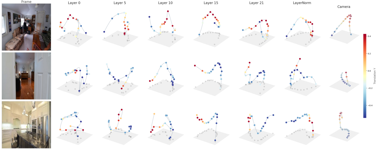
Figure 1. Layer-wise PCA projections of temporal patch representations (V-JEPA 2 L, RealEstate10K (Zhou et al., 2018)). Each row corresponds to one video clip (first frame is shown at left). Each column shows a 3D PCA projection of the 16 temporal patch features extracted from a frozen V-JEPA 2 L encoder at a specific transformer layer; each projection is computed independently per layer. Each point represents one of the 32 video frames, connected in temporal order. Points are coloured by the camera’s vertical translation ( y ) at the corresponding timestamp, with red indicating positive and blue indicating negative values. The rightmost column shows the ground-truth camera trajectory for reference. For all videos, while earlier layers contain less structure, deeper layers show geometric curves and smooth colour transitions as the ego-motion changes in the Y -axis direction.
