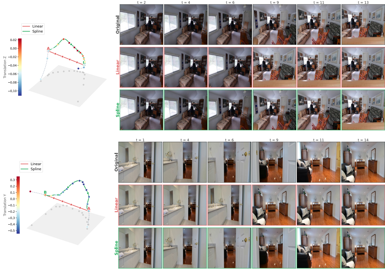
Figure 5. Nearest-neighbour evaluation of representation-space steering for V-JEPA 2 L, RealEstate10K (Zhou et al., 2018). Each row shows one video clip. The leftmost panel in each row displays the per-frame representation trajectory in 3D PCA space, coloured by camera translation ( z -axis in the top row, y -axis in the bottom row). Two temporal anchor frames A and B are selected, and the representation space between them is traversed via linear interpolation (red) or spline/tangent steering (green); the original trajectory is shown in grey for reference. The remaining panels show the nearest-neighbour video frames retrieved for each steered representation at a set of intermediate timesteps t , allowing visual inspection of whether the steered path better aligns with the underlying scene and motion dynamics. Additional 3D visualizations and steering playback are available at https://vid-rep-pca.netlify.app/ .
