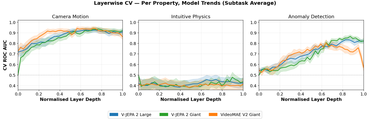
Figure 3. Probing Results. Each plot shows the average cross-validation ROC-AUC across subtasks as a function of normalised layer depth (0 = first layer, 1 = last), for three models: V-JEPA 2 Large (blue), V-JEPA 2 Giant (green), and VideoMAE-V2 Giant (orange). Shaded bands denote \pm 1 std across subtasks. The dashed line marks the chance level (0.5). Higher values indicate that a linear probe trained on that layer’s representations can better discriminate the property in question. We see Camera Motion is largely separable at early layers, Anomaly Detection peaks at deep layers, while Intuitive Physics is not encoded throughout the model. Per-property layer-wise curves for all individual subtasks are provided in the Appendix.
