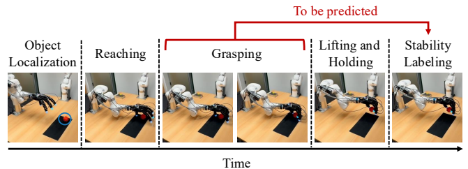
Fig. 5: Automated self-supervised data collection timeline. Each trial comprises object localization, randomized reaching and grasping, lifting, and stability labeling from object height changes, with continuous multimodal recording.
