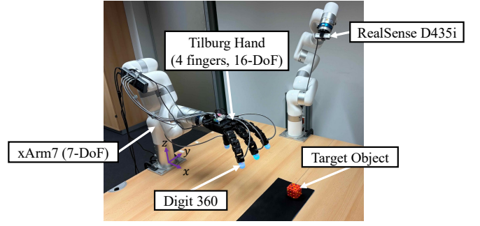
Fig. 2: Hardware setup. The system continuously records external visual observations, proprioception, and tactile streams from four Digit 360 sensors throughout each grasp trial.
