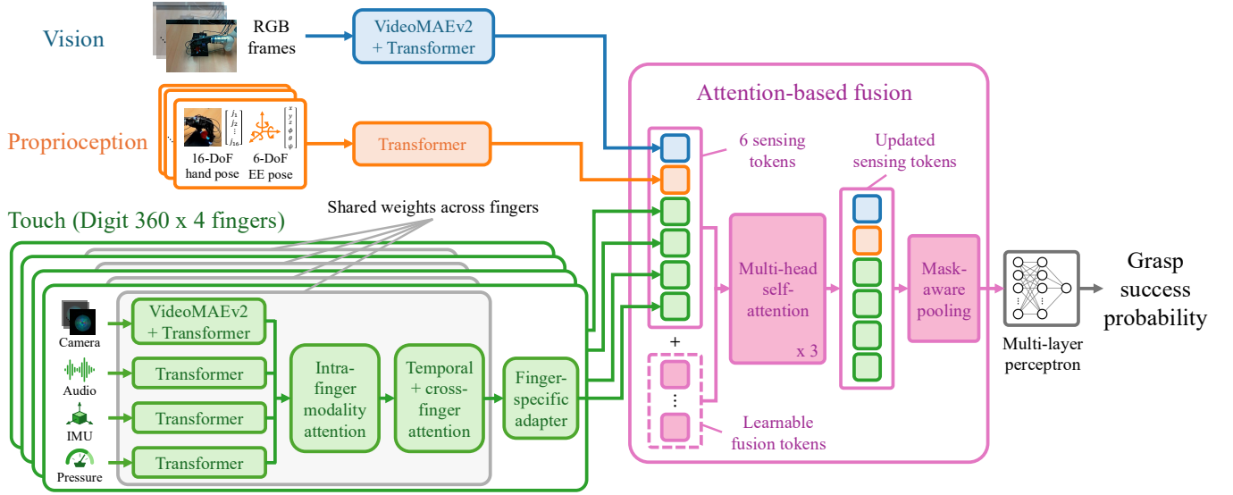
Fig. 3: Model architecture for temporal multimodal grasp stability prediction. An observation window from the pre-lift grasp phase, containing RGB frames, proprioception, and tactile streams from four Digit 360 sensors, is encoded by modality-specific Transformer-based branches. Finger-level tactile features are integrated across modalities, time, and fingers, then combined with RGB and proprioceptive features through attention-based fusion to predict post-lift grasp stability.
