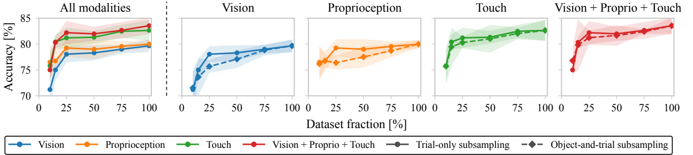
Fig. 7: Mean accuracy with SD shading across data scales for VideoMAEv2-based models. Trial-only subsampling (solid) reduces trials per object while retaining the object set; object-and-trial subsampling (dashed) also reduces the number of objects by the same ratio. The leftmost panel compares modalities; the others compare subsampling protocols. Accuracy generally improves with more data, while touch-enabled models remain comparatively robust to reduced object coverage.
