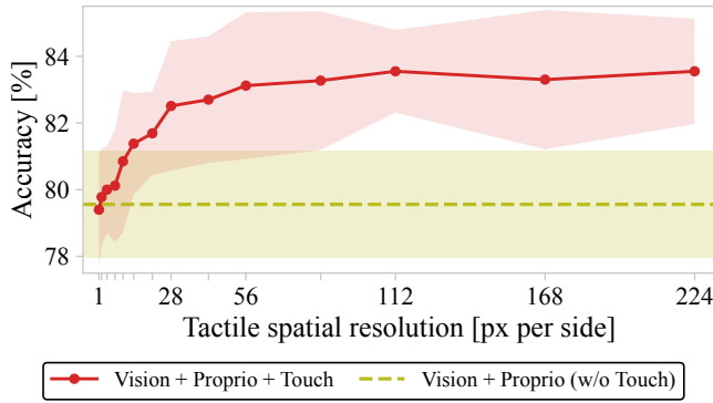
Fig. 8: Mean and SD of accuracy across tactile-image spatial resolutions, with the non-tactile baseline shown as a horizontal band. Higher tactile resolution improves accuracy.
