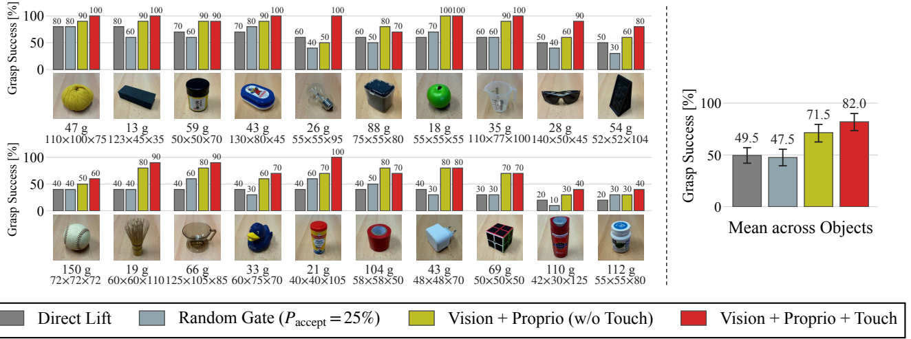
Fig. 11: Grasp success rates among executed lifts for four policies on 20 unseen objects. Object mass and dimensions ( W \times D \times H in mm) are shown below each image. The vision–proprioception–touch gate outperforms the vision–proprioception gate, direct lifting, and the random gate by 10.5, 32.5, and 34.5 percentage points, respectively. Error bars show object-cluster bootstrap 95% confidence intervals for overall success rates; per-object rates are based on 10 executed lifts per policy.
