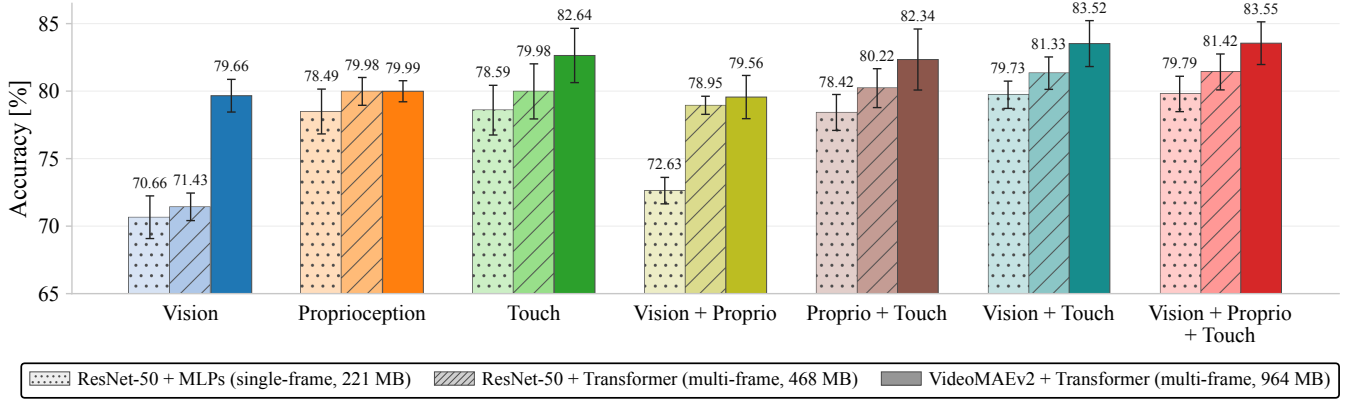
Fig. 6: Mean accuracy with SD error bars for modality and backbone ablations under 5-fold CV. Touch-enabled models achieve the strongest performance. Multi-frame models consistently outperform the static single-frame baseline, with the VideoMAEv2-based model performing best, suggesting the value of expressive temporal models for capturing grasp dynamics.
