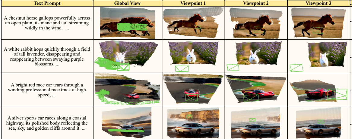
Figure 2. Qualitative results of Streaming4D. Driven purely by text prompts, our block-wise AR generator and continuous 3D reconstructor operate synchronously to model dynamic scenes. The Global View reveals the underlying 3D point cloud structure and the camera poses (green boxes) tracked over time. The Viewpoints illustrate the framework’s ability to provide geometrically grounded visual synthesis across different viewing angles and timesteps.
