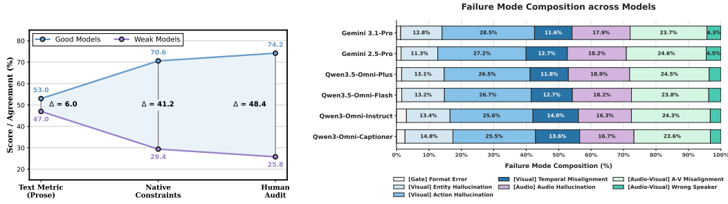
(a) The illusion of global scores. Text metrics reward fluent but flawed outputs; structured metrics expose them. (b) Failure composition. Distribution of structural errors, normalized by each model's total failures.
