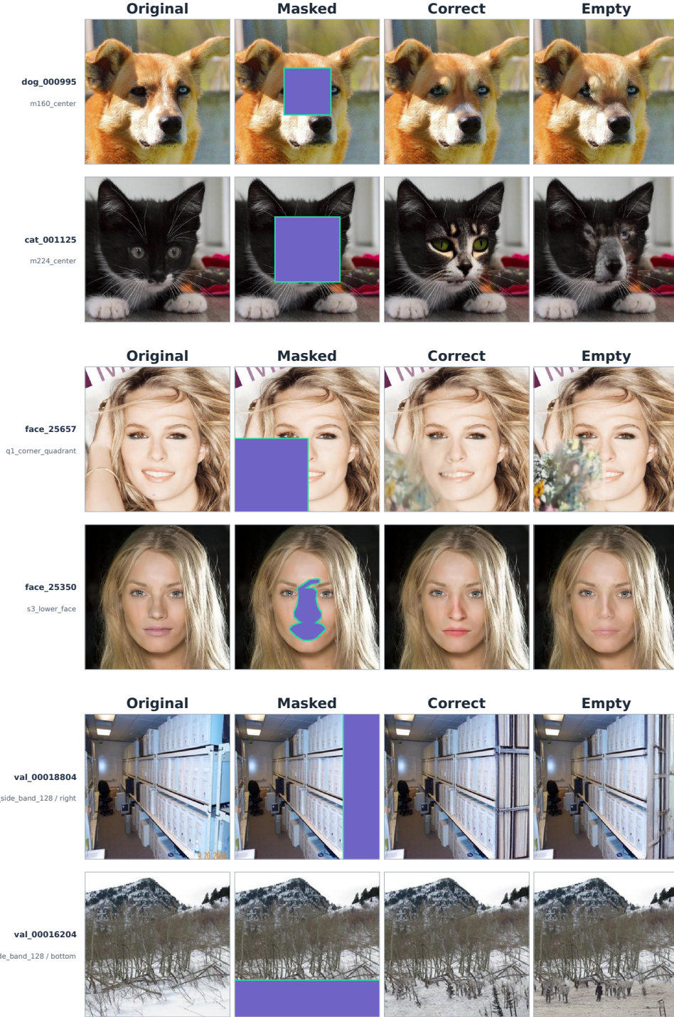
Figure 7. Prompt-presence responses on six strict-random cases: AFHQ (top), CelebA-HQ (middle), and Places2 (bottom), with two cases per dataset. Every panel uses the shared four-column order Original, Masked, Correct, and Empty. Original is evaluation-only reader context and was unavailable during inference; Masked uses the shared violet/mint display convention; and only the positive text condition differs between Correct and Empty. The corresponding aggregate and per-dataset estimates are reported in Appendix C; this plate is their strict-random visual companion.
