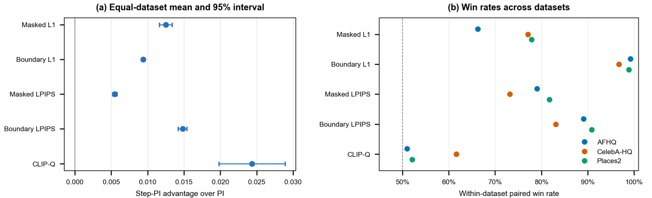
Figure 4. Paired Step-PI advantages over PI on Main35: (a) direction-normalized equal-dataset paired means with 95% case-within-protocol bootstrap intervals; (b) within-dataset paired win rates across the same five metrics. Positive values favor Step-PI; the dashed line marks 50%; all 3,500 cases contribute.
