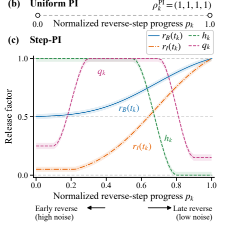
Figure 3. Stateful boundary–interior action and release. (a) Both feedback branches and persistent states update at every step; release modulates their contributions before the shared nonlinear safeguards. (b) PI uses uniform release. (c) Step-PI uses the four predefined fields of its release schedule along the reverse trajectory.
