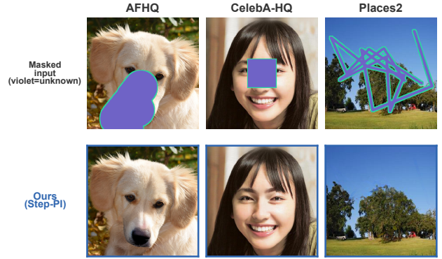
Figure 1. Three-domain conditional inpainting with frozen SD1.5. The same configuration-locked Step-PI controller is applied to an outcome-independent random sample spanning AFHQ, CelebA-HQ, and Places2, without weight updates or learned inpainting-specific conditioning channels. Text conditions are fixed before inference. Opaque violet denotes unknown pixels, and the mint contour is display-only.
