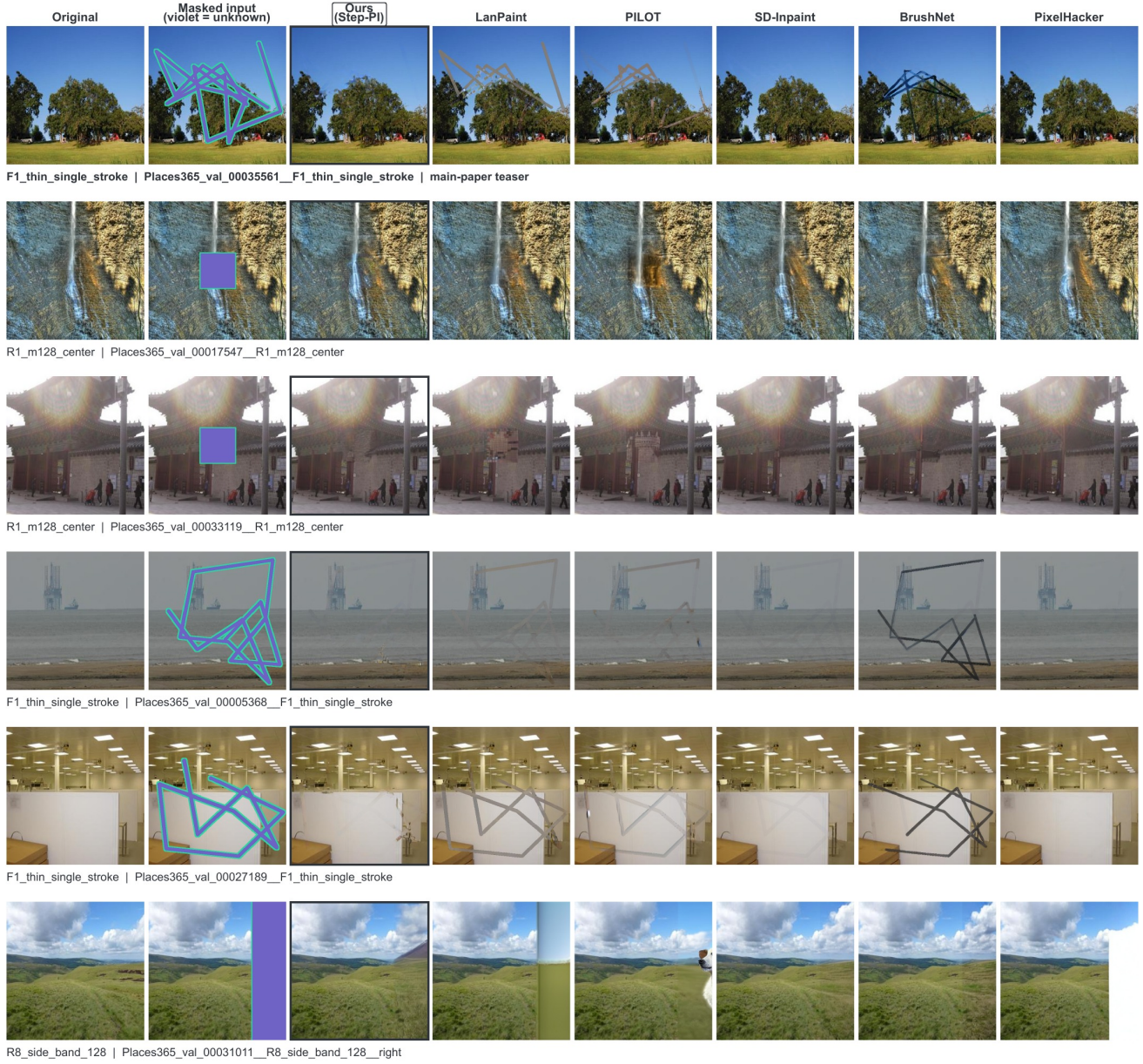
Figure 10. Native-route comparison on six randomly drawn Places2 cases. Each method receives the same image and mask within a row while retaining its native inference route, and exact identifiers are printed per row.
