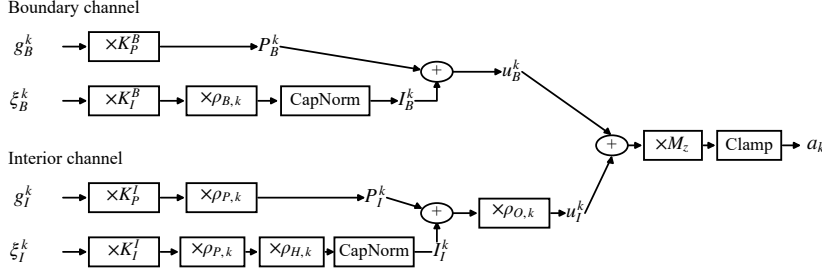
(a) Shared PI action assembly
