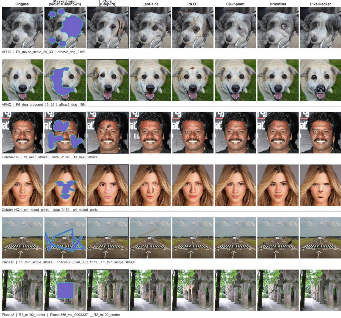
Figure 11. Cross-domain stress-test diagnostics, with two cases each from AFHQ, CelebA-HQ, and Places2 and the complete active comparison lane retained for every case. Horizontal rules separate datasets, and exact protocol and case IDs are printed below every row. The plate supports inspection of challenging structural, semantic, and blending behaviors rather than prevalence estimation or causal attribution.
