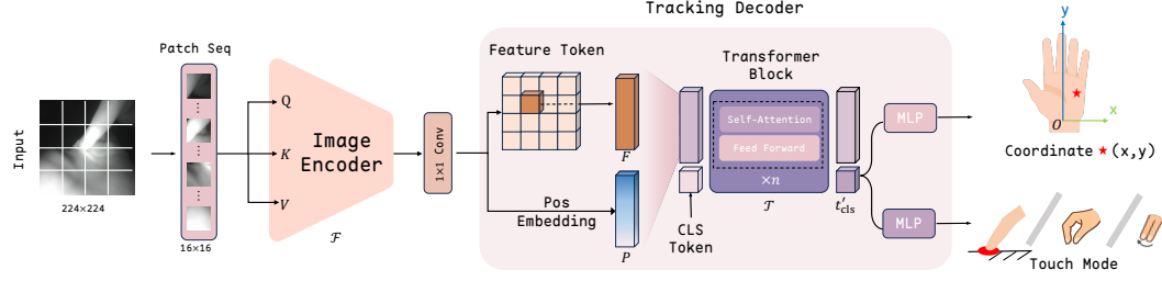
Fig. 4. PalmSpace network architecture.
