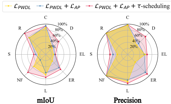
Figure 8: Loss term ablation for Phase 3 with MixedWM38. The left figure compares mIoU across single-type defect patterns, and the right depicts the difference in Precision.
