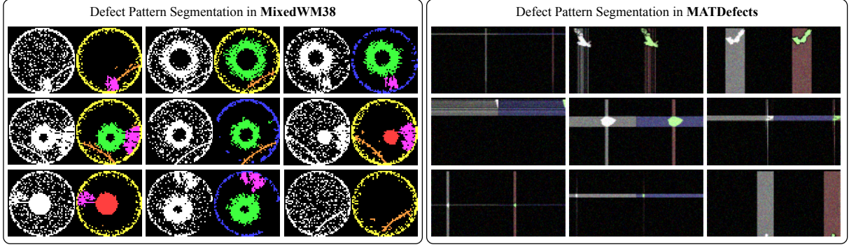
Figure 7: Examples of segmented defect pattern in test images, using our proposed method, SePArate. For proprietary reasons, the examples of MATDefects were slightly modified from the original data. Key patterns were preserved regardless of modification.
