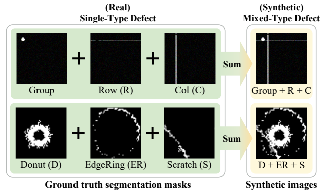
Figure 5: Generation of synthetic mixed-type defect images.
