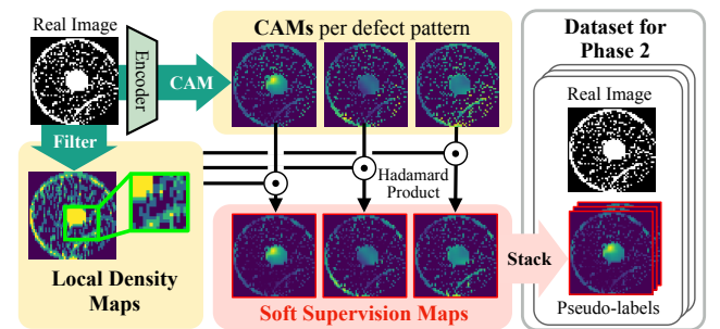
Figure 4: Generation of soft supervision maps. For each image, local density map (bottom left) and CAM (top center) are computed, combined to generate soft supervision maps.
