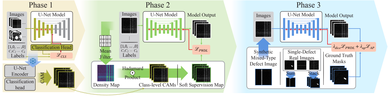
Figure 3: A full overview of our proposed method, SePArate. i) Phase 1 trains the encoder for multi-label classification, enabling the model to learn about defect patterns using image-level labels. ii) Phase 2 transfers classification knowledge to the U-Net by training with soft supervision maps and pattern-weighted Dice loss. iii) Phase 3 further tunes the model using synthetic mixed-defect data, improving precision with pattern-weighted Dice loss and absence-penalty scheduling.
