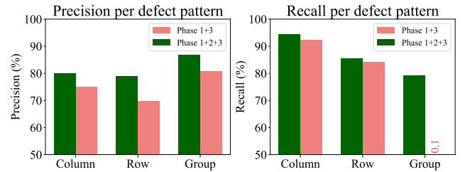
Figure 6: Precision and Recall comparison with and without Phase 2 in SePArate, with MATDefects. It shows improved metrics when trained using all 3 phases.
