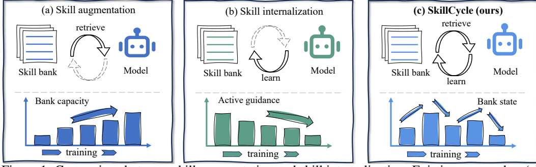
Figure 1: Comparison between skill augmentation and skill internalization. Existing approaches (a) augment the policy with an external skill bank or (b) internalize skills into the policy to reduce reliance on external guidance. (c) Our proposed SkillCycle couples skill internalization with evidence-driven skill-bank revision, co-evolving the policy and the bank for skill-free inference. Bars and arrows illustrate conceptual trends, not measured trajectories.
