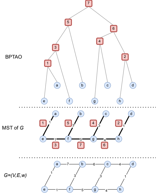
Fig. 4 A weighted graph G = (V, E, w) , a MST of G with a non-decreasing ordering on its edge weights indicated in red, and the BPTAO of this MST for this given ordering.
