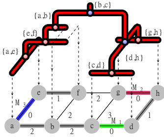
Fig. 7 Unsupervised watershed cut. The underlying graph has 3 minima: edges M_1 (green), M_2 (red) and M_3 (blue). By applying Algorithm 6 to the BPTAO where one vertex of each minimum is seeded, we can identify the watershed nodes (blue points) and their associated MST edges \{b, c\} and \{d, h\} .
