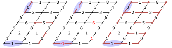
Fig. 2 Left: an initial edge-weighted graph with three minima in bold red and two seeds overlaid in blue. Middle: a closing by reconstruction from the initial graph and the seeds (changed weights in red). Edge weights within seeds are set to -1, forcing them to become minima. The closing by reconstruction then fills the minima of the original graph. Finally, the associated watershed cut is depicted by dashed edges. Right: a minimum spanning forest (bold red) of the initial graph rooted in the seeds, together with its induced graph cut (dashed edges), which coincides with the watershed of the closing by reconstruction in the middle figure, as stated in Theorem 3.
