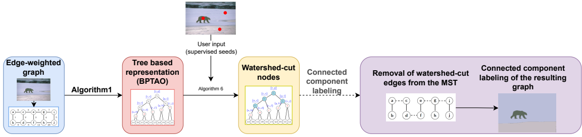
Fig. 10 Seeded watershed-cut pipeline.
