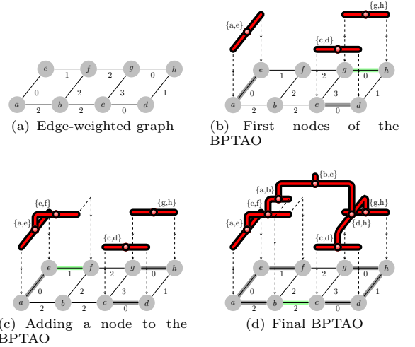
Fig. 6 Some steps of the construction of the MST of an edge-weighted graph with Kruskal's algorithm and the corresponding BPTAO. Top left: initial edge-weighted graph: each vertex of the graph represents a region. Top right: the algorithm first processes the edges \{a, e\} , \{g, h\} and \{c, d\} of weight 0 in any arbitrary order. The vertices corresponding to those edges are merged: this is represented by the red trees whose root nodes indicate the edge of the MST where the merge occurred. Bottom left: then the edge \{e, f\} is processed. The region \{a, e\} is merged with the singleton \{f\} . Bottom right: the process continues until the edge \{b, c\} is processed, completing the MST and leading to a partition with a single region containing all the vertices.
