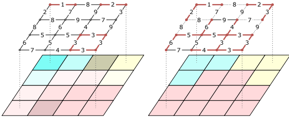
Fig. 1 Left: A digital image (bottom) and an edge-weighted graph representing this image (top): vertices correspond to pixels and edges represent the adjacency between pixels. The edge weights measure the dissimilarity between the values of adjacent pixels. The three minima of the edge-weighted graph are represented in bold red. Right: a watershed cut of the edge-weighted graph, which is represented by dashed edges in the graph (top) and by a color label in the image domain (bottom). The minimum spanning forest rooted in the minima of the graph associated to the watershed is depicted in bold red.
