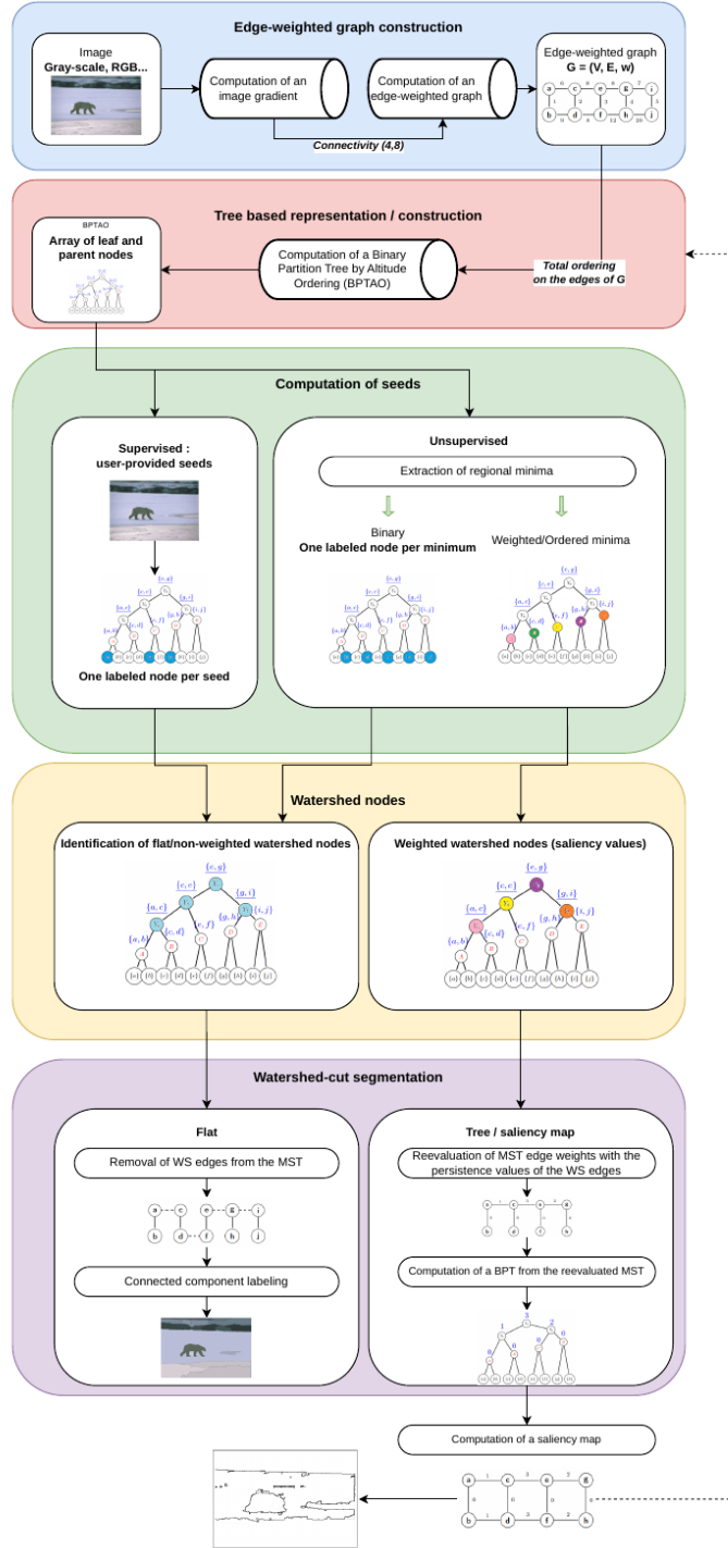
Fig. 5 Algorithmic overview of (hierarchical) watershed-cut segmentation.
