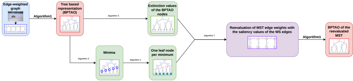
Fig. 12 Pipeline for computing a tree representation of a hierarchical watershed.
