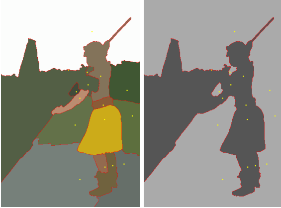
Fig. 11 The image and gradient considered are the same as in Figure 9. The user provides two sets of pixels as seeds: a set of foreground seeds and a set of background seeds. On the left is the supervised watershed cut. Each region is filled with its average color, and the contours are drawn in red. Each region contains a single yellow point depicting the location of its associated seed. Right: the final segmentation obtained by grouping the regions associated with the foreground and background seeds. It can be seen that the contours are well placed overall with a small number of seeds; however, a gradient leak on the person's shoulder causes a large error.
