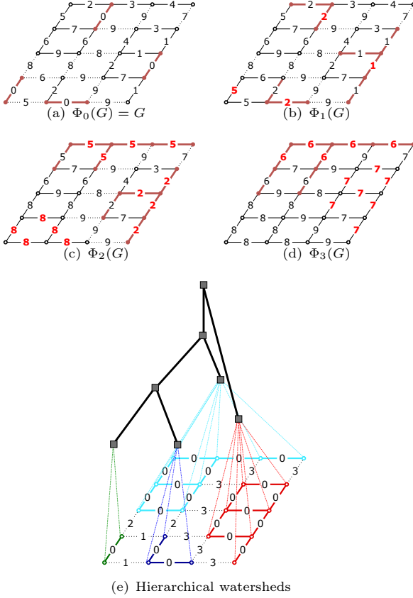
Fig. 3 (a-d): Four filtrations of a graph obtained with a connected closing by area removing successively the components with less than 0, 3, 6, and 8 vertices. The edge weights that changed between two levels of filtrations are highlighted in red. The minima are in bold red. The watershed cuts of each filtration are represented by dashed edges. Observe that the watershed cut obtained at one filtration level is included in the watershed cut obtained at a lower level. (e): The watershed cuts of the series of filtrations form a hierarchical watershed. It can be represented as a saliency map (bottom), i.e., an edge-weighted graph, where the weight of an edge indicates at which filtration level it ceases to be in the cut or 0 if it does not belong to any watershed cut. Note that every watershed cut from the series of filtration can be recovered by thresholding the saliency map. The four regional minima of the original graph are the four minima, all at level 0, of the saliency map (each depicted in a different color). The hierarchical watershed can be equivalently represented as a tree (top) representing the fusion of regions along the filtration process.
