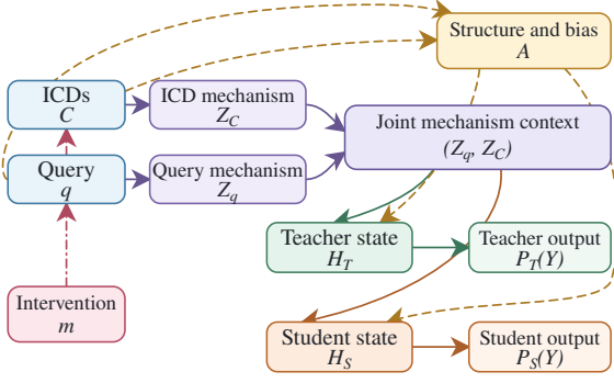
Figure 2: Causal graph of multimodal ICL inference. The query and ICDs provide complementary mechanism evidence and jointly shape the model state.
