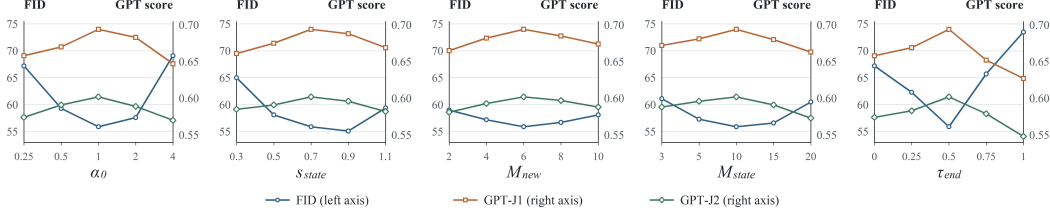
Figure 3: Sensitivity analysis for hyper-parameters of SCO ( \alpha_0 , s_{state} , M_{state} , M_{new} , and \tau_{end} ).
