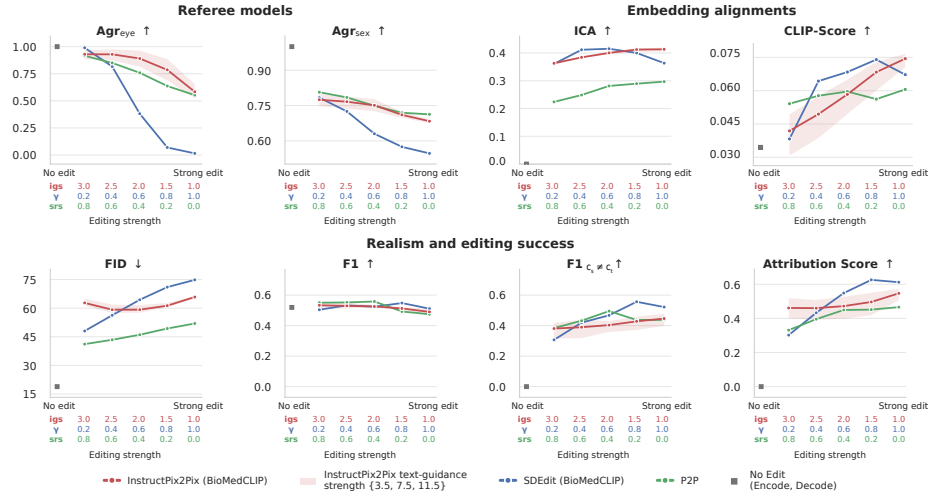
Fig. 4. With increasing editing strength, all investigated text-conditioned editing strategies show a loss in identity preservation, most prominently revealed by \text{Agr}_{\text{eye}} , \text{Agr}_{\text{sex}} . Above all, we find that even minor edits can cause a drastic loss of identity features, which is not equally compensated by gains in editing success metrics.
