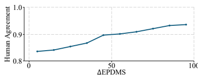
Fig. 6: Human agreement relative to EPDMS difference. Larger \Delta EPDMS yields stronger agreement.
