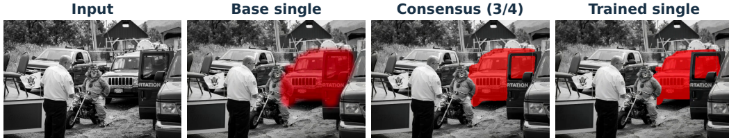
Figure 4: Referring-segmentation outputs for the prompt “jeep just to right of clown”. Base and trained single-generation panels show final frames with the same seed. The consensus panel visualizes a three-of-four vote over the base model’s extracted masks; all outputs use early readout. The trained panel uses the model after consensus RFT from Table 2.
