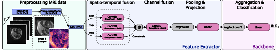
Fig. 2: STORK network architecture composed of a preprocessing stage (green), a feature extractor (blue) and backbone (pink). Preprocessing stage transforms each series into a 4-channel input combining magnitude images with Demons displacement fields. The feature extractor processes the 4D volume by leveraging 3D convolutions on hyperplanes always involving the temporal dimension. The backbone aggregates information over the time dimension by average pooling combined with a linear projection.
