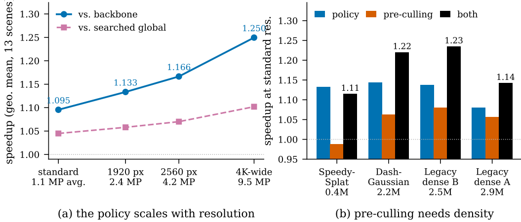
Figure 5: Each mechanism has a regime, and the cost model names it. (a) The compiled policy strengthens with resolution; both P and |\Omega| change in this sweep. The separate stage profiles in Figure 4 show the within-scene changes and do not conflate the bicycle and counter endpoints. (b) Pre-culling strengthens as the measured aN/T share grows. The dense bars are stress-test checkpoints; the two legacy packaged checkpoints are not used as evidence for any named model family. On Speedy-Splat’s 0.4M checkpoint the frustum test costs more than it saves and “both” is worse than the policy alone, which is the case the dispatch rule catches.
