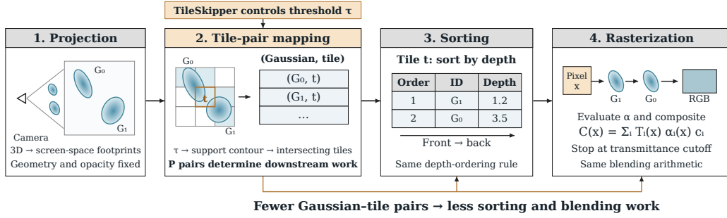
Figure 2: TileSkipper changes pair enumeration at stage 2. The blue and orange outlines denote support under the baseline and compiled cutoffs. Tiles excluded by the compiled support generate no Gaussian–tile pair and therefore enter neither sorting nor blending. For tile t , the figure shows the resulting depth order and compositing expression; T_i is transmittance before contribution i .
