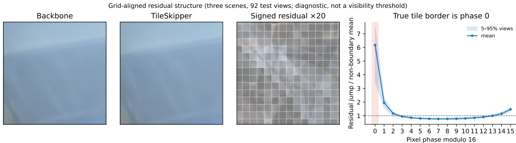
Figure 8: Grid-aligned residual diagnostic. The crop is selected by maximum boundary-weighted residual energy and the signed residual is amplified 20\times ; white lines show the true tile grid. The phase plot pools the Regional policy over three scenes and 92 test views. The highlighted phase zero is the actual tile border. The plot diagnoses residual structure and is not a perceptual visibility threshold.
