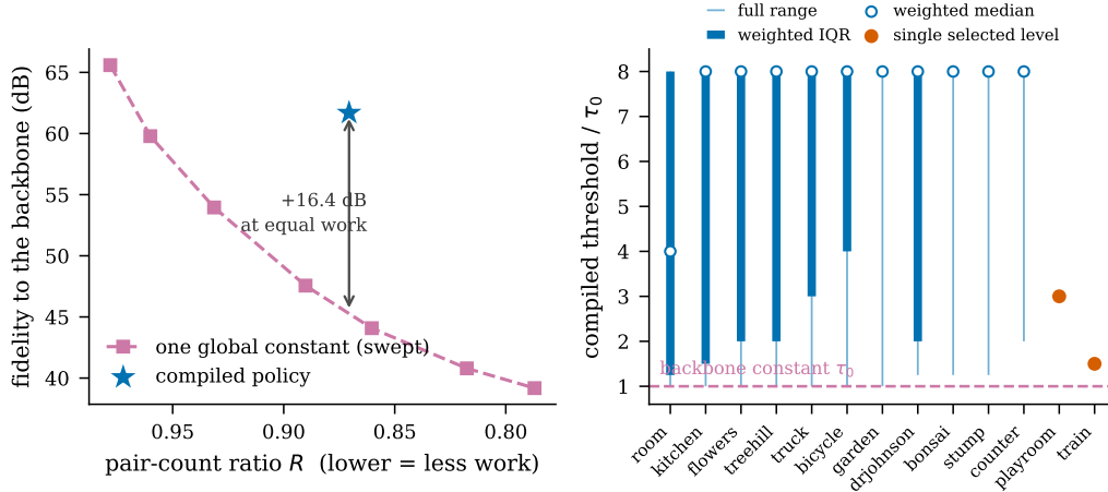
(a) the constant traces a curve the policy is not on (b) and the compiled answer is usually spread out (flowers, the median scene by this margin) (work-weighted quantiles over 64 regions)
