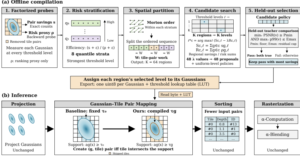
Figure 3: Offline compilation and runtime application of TileSkipper. The diagram abbreviates the region-count symbol K_{\text{reg}} as K . (a) Once per scene, the compiler uses a frozen 3DGS checkpoint and calibration views to measure per-Gaussian pair savings s and isolated-removal risk proxies \rho for each threshold level. The backward probe collects sensitivities without updating any model parameter. Gaussians are assigned to eight efficiency-quantile strata q_1, \dots, q_8 (low to high). Within each stratum, Morton ordering and workload-balanced contiguous partitioning produce K_{\text{reg}} = 64 regions in total; Gaussian counts may differ between regions. For region c and level \ell , S_{c, \ell} = \sum_{g \in c} s_{g, \ell} and R_{c, \ell} = \sum_{g \in c} \rho_{g, \ell} aggregate pair savings and risk. Each penalty \lambda selects one level for each of the K_{\text{reg}} regions. The 48 resulting proposals and uniform-level policies are rendered on disjoint held-out training views. A policy passes only if its minimum per-view teacher PSNR meets P_{\min} and its worst-view p99 absolute residual does not exceed E_{\max} ; among passing policies, the compiler selects the one with the greatest pair savings. Teacher comparisons use the unmodified backbone; p99 is computed from maximum absolute RGB-channel residuals on a fixed 4 \times spatial subsample. Test views are never used for selection. (b) Each Gaussian inherits its region’s selected level, exported as one uint8 per Gaussian plus a threshold lookup table. At inference, the default threshold is \tau_g = m_g \tau_0 , where m_g is the selected multiplier and \tau_0 is the baseline threshold. Backend-specific handling of opacity caps is described in Section E.1. The contribution field a_g(x) defines the thresholded support \{x : a_g(x) \geq \tau\} . A Gaussian–tile pair is created when the tile intersects this support, using \tau_0 for the baseline and \tau_g for TileSkipper. The dashed blue contour denotes the original support, the orange contour the compiled support, and shaded orange tiles the skipped pairs. Gaussian parameters remain unchanged. The byte and lookup table are read inside tile enumeration, with no per-frame policy inference or additional kernel; projection, sorting, and blending remain unchanged. Footprints, partitions, and table entries are schematic.
