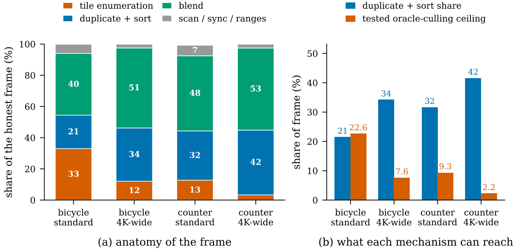
Figure 4: Measured headroom under two controlled interventions. (a) Stage shares measured with the rasterizer’s own CUDA events. (b) The mechanisms have different primary targets, but their runtime effects are not assumed to be disjoint or additive. Thresholding changes tile enumeration, duplicate/sort work, and correlated blending; pre-culling avoids processing rejected Gaussian blocks and may also change downstream work. Within each profiled scene, the duplicate-plus-sort share grows with resolution: 21.4% \rightarrow 34.2% for bicycle and 31.6% \rightarrow 41.6% for counter . The estimated ceiling of the tested perfect, free visibility culler falls from 22.6% to 7.6% and from 9.3% to 2.2%, respectively. Dispatch uses measured net benefit, including planning overhead.
