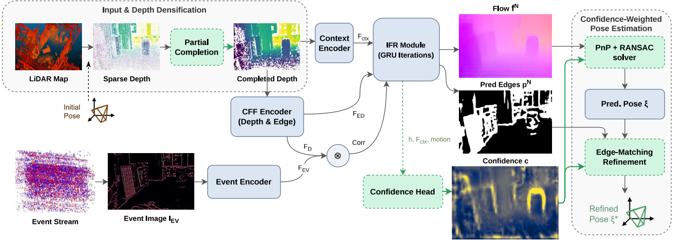
Fig. 1. Our pipeline. We extend the LEAR baseline with three components (green, dashed): a partial depth completion, a confidence head trained end-to-end through the pose loss, and a confidence-weighted edge-matching refinement . Sample maps are outputs on falcon_indoor_flight .
