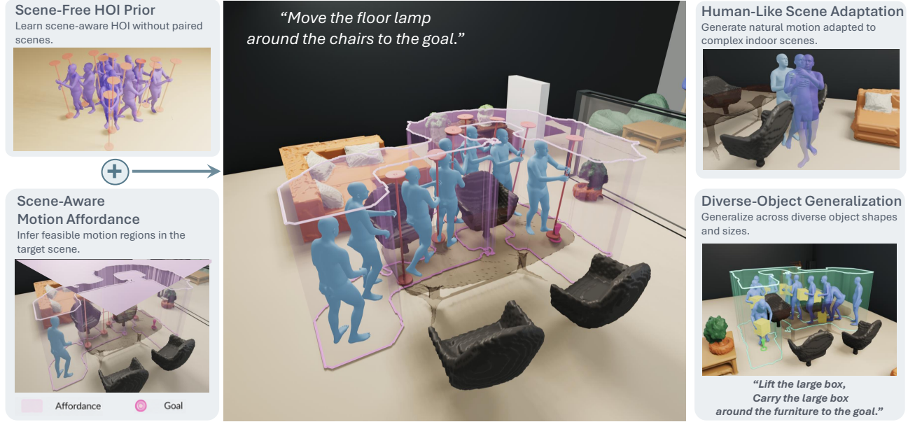
Figure 1: MAMHOI learns from Scene-Free HOI priors and transfers the ability to complex environments through scene-aware motion affordances. This factorization enables physically plausible interactions across cluttered scenes and diverse objects.
