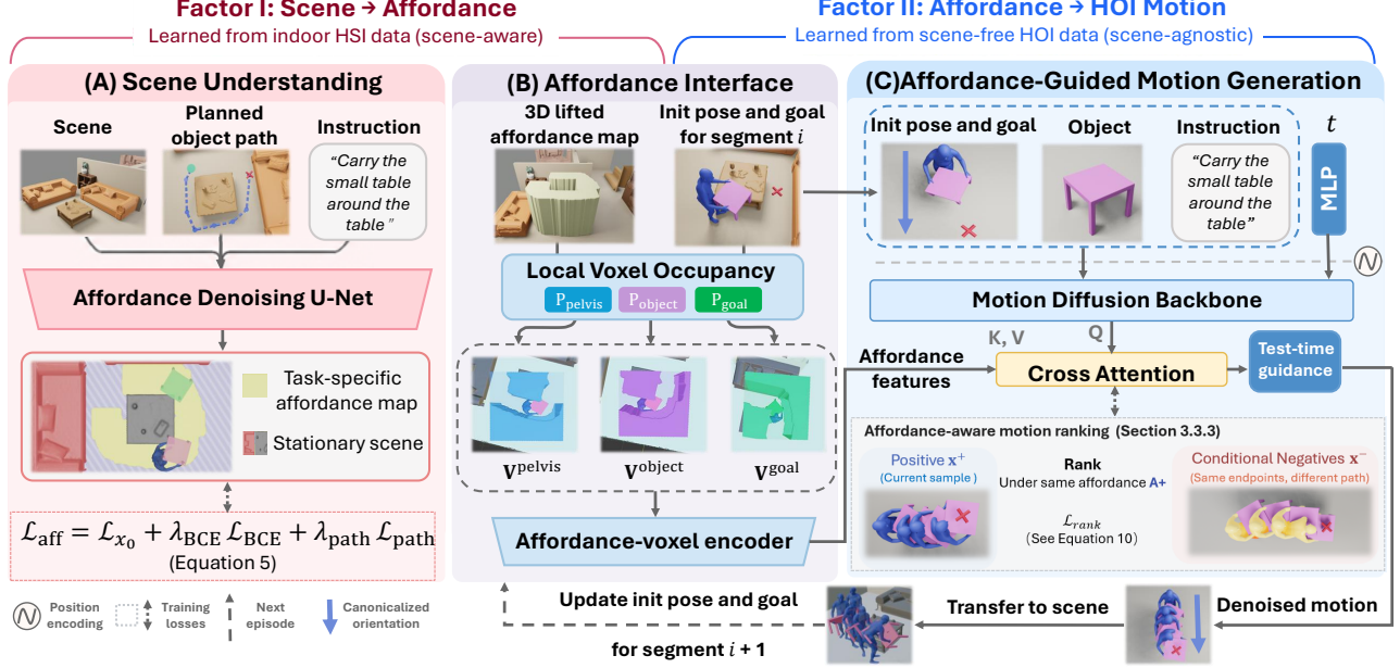
Figure 2: Overview of MAMHOI. (A) The scene-understanding module predicts a task-specific affordance from the scene, planned object path, and instruction, where the instruction guides the task-relevant human placement along the object path. (B) The affordance interface lifts the predicted affordance to 3D and queries local occupancy around the pelvis, object, and goal position of current segment, and encodes them into affordance features through a ViT-based Affordance-voxel encoder. (C) The resulting affordance features condition segment-wise HOI generation through cross-attention, with each generated segment initializing the next. Through this design, scene-aware HOI generation is factorized into a scene-to-affordance factor learned from indoor HSI data and an affordance-to-motion factor learned from scene-free HOI data.
