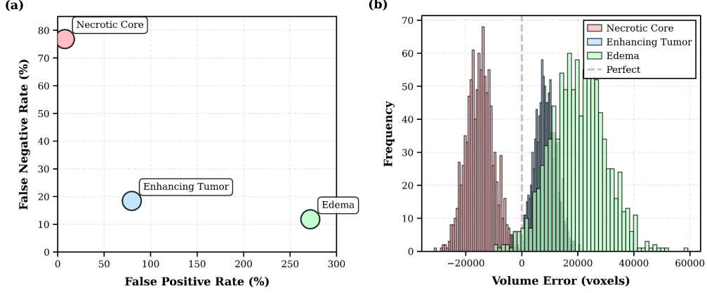
Figure 1: Class-specific error patterns revealing asymmetric biases in brain tumor segmentation, measured on the validation split. (Left) False positive versus false negative rates. Rates are normalized by ground-truth volume v^* (Eq. (5)), so values above 100% are well defined and indicate severe over-segmentation. Necrotic core shows a false-negative bias, edema a large false-positive bias, and enhancing tumor a moderate false-positive bias. (Right) Distribution of volume errors across classes, showing the skew that motivates asymmetric interval design.
