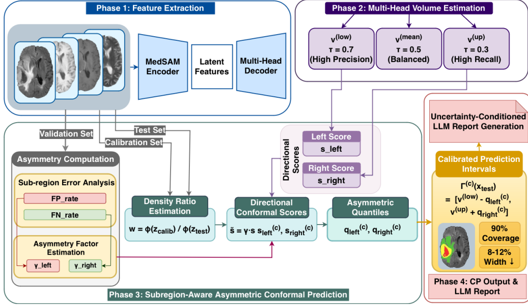
Figure 2: Overview of the proposed CA-WCP pipeline: feature extraction, multi-threshold segmentation, and weighted asymmetric conformal prediction.
