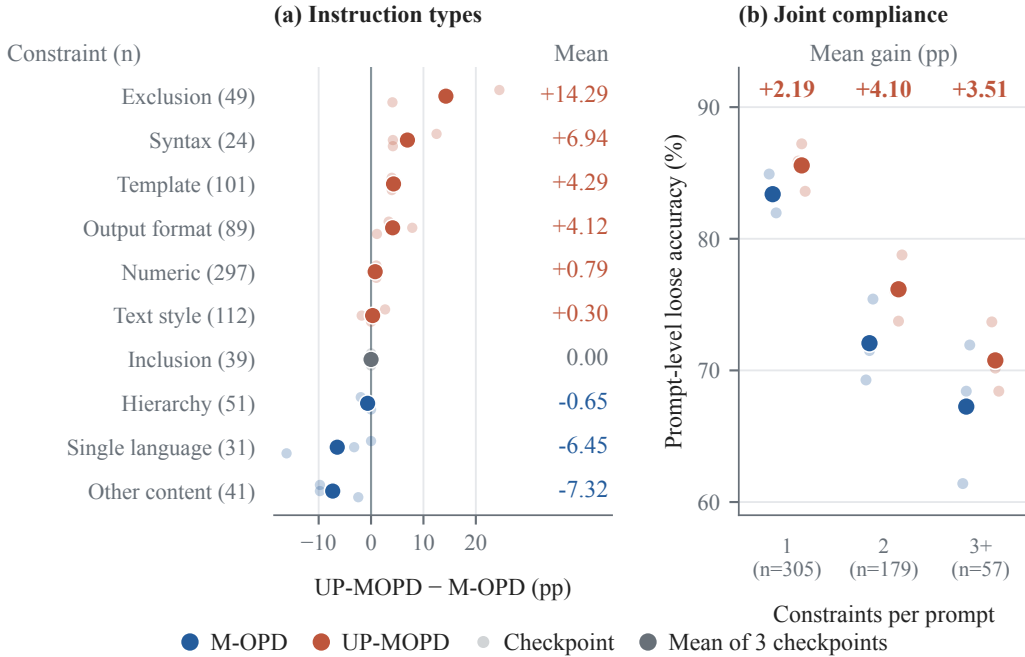
Figure 7: Instruction-following behavior in the medical setting. (a) UP-MOPD minus M-OPD instruction-level loose accuracy for all ten evaluator-defined constraint categories; parentheses give instruction counts. (b) Prompt-level loose accuracy grouped by the number of constraints in a prompt; labels above the groups give the mean gain in percentage points. Faint points show three matched late-training checkpoints from one run per method; solid points show their arithmetic mean.
