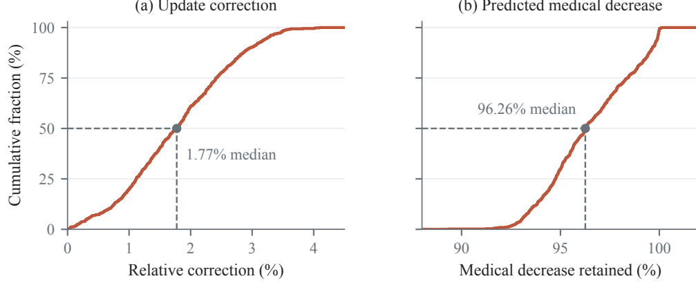
Figure 5: Offline projection of 645 rejected candidates. Cumulative distributions show relative correction size (left) and retained predicted medical loss decrease (right). Dashed lines mark medians.
