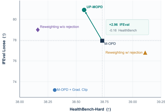
Figure 2: Medical performance and instruction following. Student points average the last three saved checkpoints of one training epoch. The arrow from M-OPD to UP-MOPD shows improved IFEval-loose accuracy at a similar HealthBench-Hard score.
