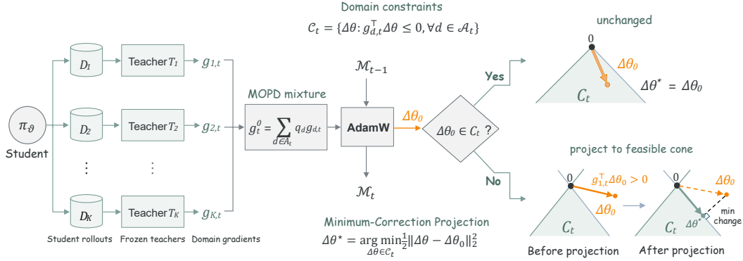
Figure 1: Overview of UP-MOPD. AdamW forms a candidate parameter displacement from the mixed distillation gradient. UP-MOPD evaluates its first-order effect on each active domain and minimally corrects a violating candidate before commit, while retaining the current-step optimizer state produced by the original mixture.
