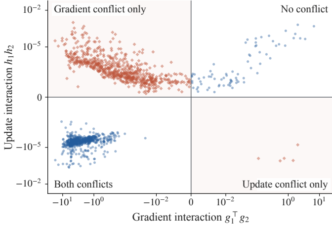
Figure 3: Gradient alignment and update conflict. Each point is a training step, with g_1^\top g_2 on the horizontal axis and h_1 h_2 on the vertical axis. A negative h_1 h_2 means the candidate update is predicted to lower one domain’s loss and raise the other’s. Gradient alignment alone does not determine this outcome.
