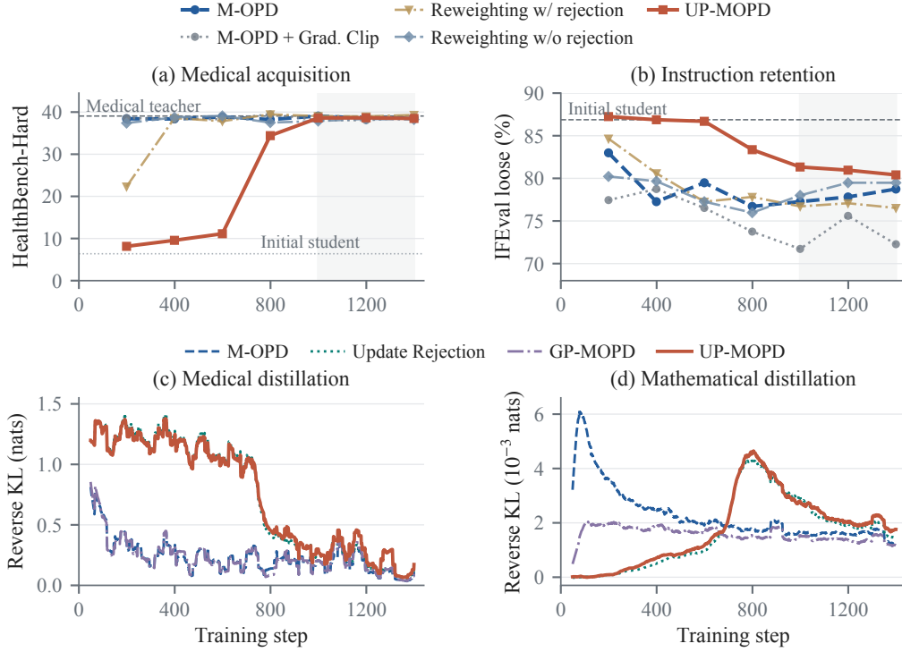
Figure 4: Capability and distillation dynamics. (a,b) HealthBench-Hard and IFEval-loose checkpoint scores; lines denote teacher or initial-student references and shading the late-training window. (c,d) Trailing 50-step means of domain-conditioned sampled reverse KL on each method’s responses; steps lacking a domain and incomplete initial windows are omitted.
