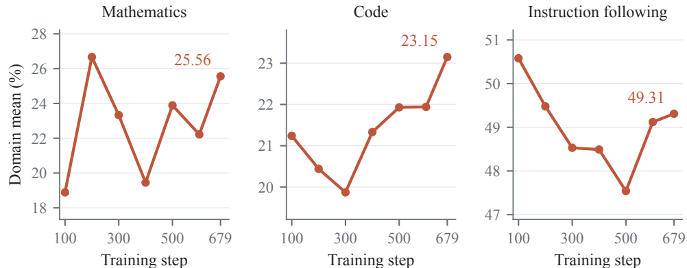
Figure 6: UP-MOPD training trajectory in the public three-domain setting. Each panel shows a domain mean over two benchmarks. The vertical scales differ across panels.
