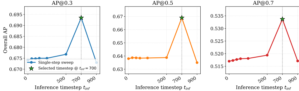
Figure 8: Sensitivity to the single-step inference timestep t_{\text{inf}} on DAIR-V2X under 90% packet loss. Solid curves show sweep results from a fixed checkpoint across different t_{\text{inf}} values, and the star marks the selected timestep t_{\text{inf}} = 700 . The trend is broadly stable across timesteps, indicating that the single-step denoiser is not highly sensitive to the exact inference timestep within a wide operating range.
