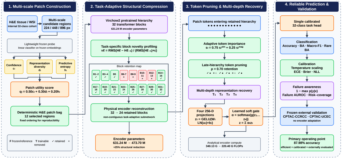
Figure 3: Architecture of the proposed TAP-Path framework. Multi-scale H&E regions are ranked to construct a deterministic 12-patch bag, followed by task-adaptive structural compression of the Virchow2 encoder to the locked one-based block set \{1, \dots, 5\} \cup \{14, \dots, 32\} (24 of 32 blocks). Adaptive late-hierarchy token pruning retains 70% of informative tokens, while four intermediate feature representations are projected to 256 dimensions and adaptively combined through a learned soft gate before 32-class prediction. The resulting predictions are evaluated for classification performance, calibration, failure awareness, and frozen external generalization on CPTAC-CCRCC and CPTAC-UCEC. TAP-Path reduces the encoder from 631.24M to 473.70M parameters and the analytical encoder computation from 340.13 to 220.40 GFLOPs while achieving 87.98% internal test accuracy.
