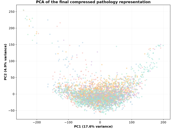
Figure 13: PCA of held-out TAP-Path image-level representations.
