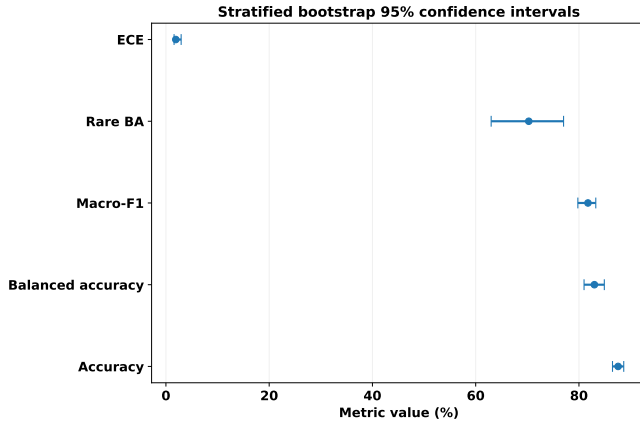
Figure 14: Stratified 95% bootstrap confidence intervals for the locked TAP-Path test evaluation.
