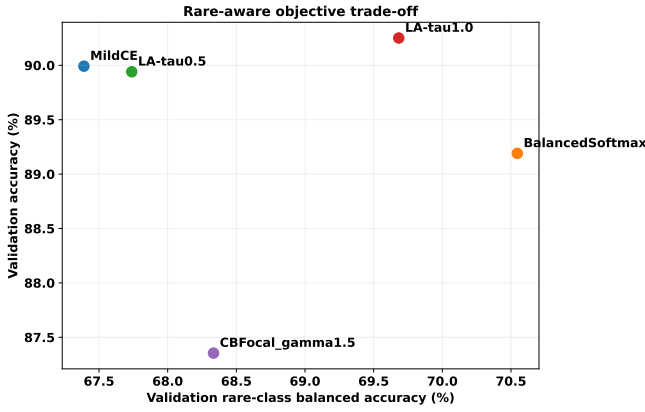
Figure 10: Validation trade-off between overall accuracy and rare-class balanced accuracy for alternative task-head objectives on the fixed TAP-Path encoder.
