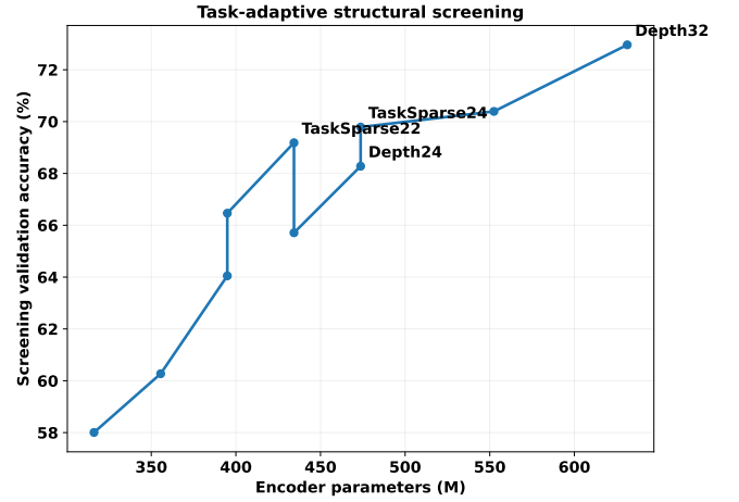
Figure 4: Validation-only structural screening of contiguous-depth and task-adaptive sparse candidates.
