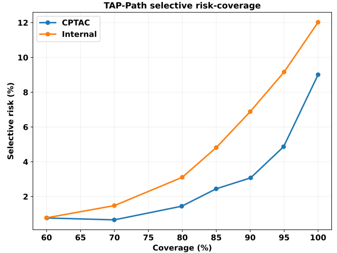
Figure 9: Selective risk–coverage behavior for TAP-Path on the locked internal and external evaluations.
