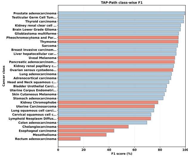
(a) Per-class F1. Rare classes are highlighted with the contrasting bar color.
