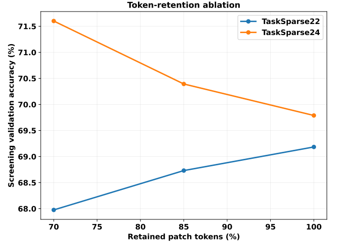
Figure 5: Token-retention ablation after structural selection. The 70% TaskSparse24 configuration provides the best validation accuracy with the lowest compute among the displayed TaskSparse24 settings.
