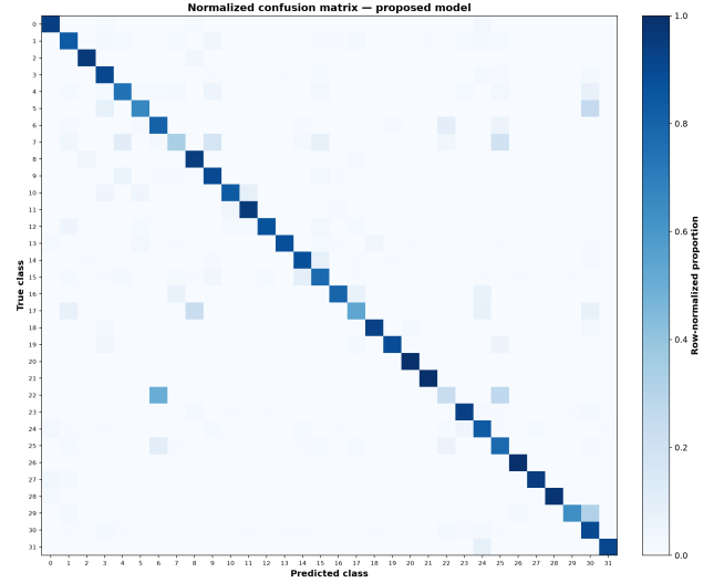
(b) Row-normalized 32-class confusion matrix.
