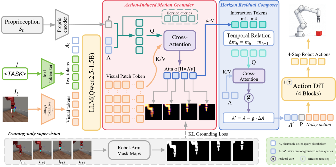
Fig. 1. Overview of MotionWeave. The current observation I_t and instruction l are tokenized into visual tokens and text tokens, concatenated with a learnable action query placeholder A_0 , and jointly processed by LLM to produce action tokens A ; a separate proprioceptive encoder maps S_t to P . The Action-Induced Motion Grounder (AIMG) combines A and P into horizon-specific queries that attend over visual tokens V to produce interaction tokens M with spatial attention \alpha . The Horizon Residual Composer (HRC) injects adjacent-horizon differences of M into A via gate g to obtain A' , decoded by Action DiT into a 4-step chunk. Robot-arm masks [10] supervise \alpha via KL loss in training only.
