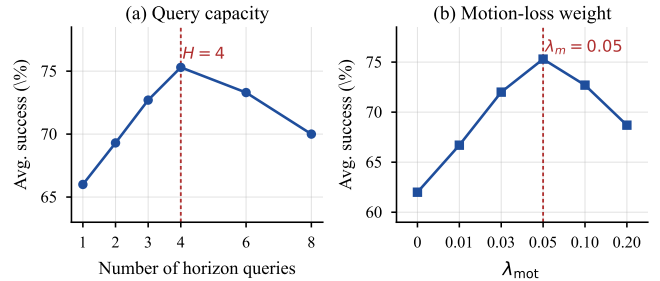
Fig. 3. Hyperparameter curves in average success (%). (a) Horizon query count peaks at 4 with 75.3%, aligned with the action chunk length H = 4 , falling back to 73.3%/70.0% at 6/8 queries. (b) Motion loss weight \lambda_{\text{motion}} peaks at 0.05 with 75.3%, falling back to 72.7%/68.7% at 0.10/0.20.
