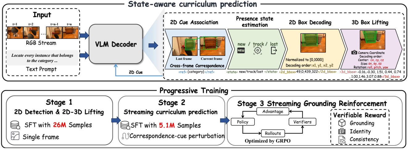
Figure 2: TempoGround overview. Top: state-aware curriculum prediction guided by cross-frame correspondence, consuming adjacent dual-image frames with the language query and previous 2D cue, from presence-aware 2D localization to camera-frame 3D lifting. Bottom: progressive three-stage training from single-frame SFT to streaming curriculum prediction and Streaming Grounding Reinforcement (SGR).
