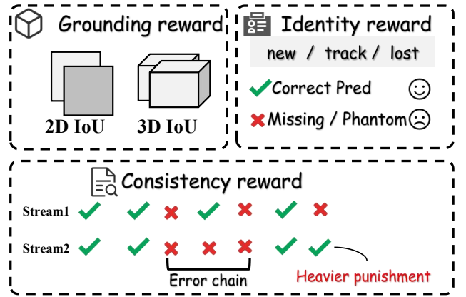
Figure 3: Verifiable rewards in SGR.
