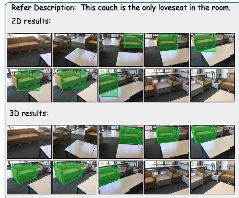
Figure D.4: TempoGround interprets the query “loveseat” and correctly identifies the two-seat couch in the view, avoiding false detections of single-seat or three-seat ones.
