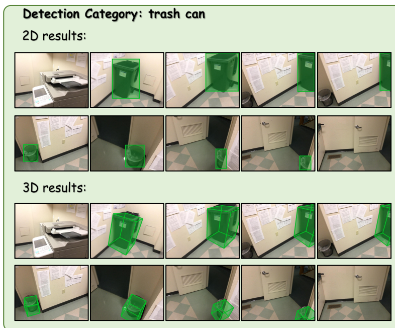
Figure D.2: The scene contains both a large and a small trash can; TempoGround accurately detects the two instances.
