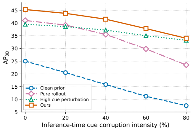
Figure 4: Closed-loop robustness to inference-time cue corruption on ScanNet (AP 3D ).
