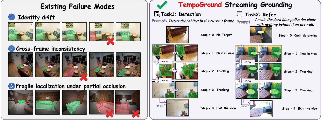
Figure 1: TempoGround for streaming visual grounding. Under streaming inputs, visual grounding commonly exhibits three characteristic failure modes (left). By exploiting cross-frame correspondence for state-aware curriculum prediction, TempoGround yields more stable camera-frame 2D/3D localization under streaming inputs (right) for both detection and referring grounding.
