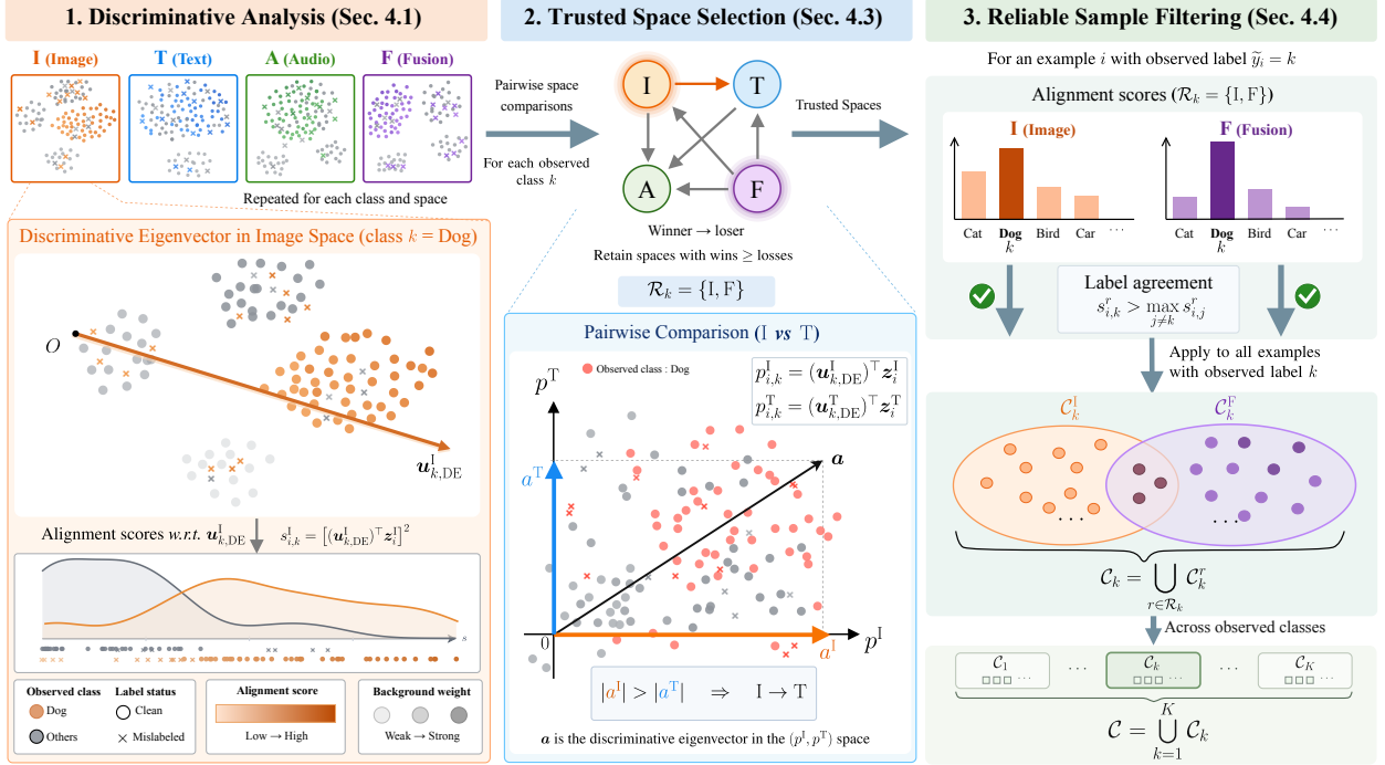
Figure 2: The overall framework of the proposed REFINE. ( Part 1 ) We construct discriminative eigenvectors for each class in the fused and unimodal spaces through discriminative analysis of the target and background. ( Part 2 ) We select trusted spaces with stronger noise detection ability for each class through pairwise comparisons across spaces. ( Part 3 ) We select reliable examples based on their alignment with the discriminative eigenvectors in each trusted space and take the union of the selected subsets.
