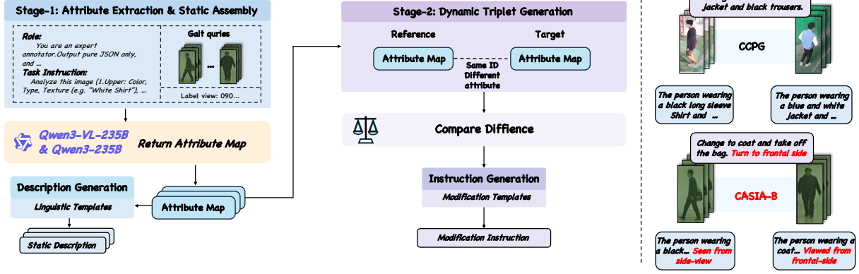
Figure 2: The automated VLM-based dataset construction pipeline. The first two stages extract fine-grained visual attributes and assemble static descriptions. Reference and target tracklets of the same identity are then compared to identify changed attributes and synthesize relative instructions. Language-Augmented CASIA-B includes explicit viewpoint shifts, whereas Language-Augmented CCPG focuses on appearance changes to reflect the structure of each dataset.
