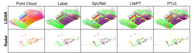
Fig. 7: LiDAR and Radar experiments (see Section VII-C).
