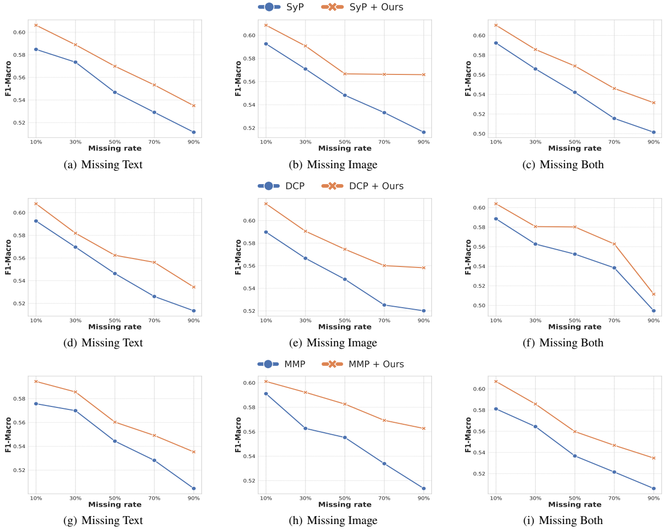
Figure 4: Plug-and-play evaluation of TLP with existing missing-modality methods on MM-IMDb (Arevalo et al. 2017). MMP (Lee et al. 2023), DCP (Hu et al. 2024), and SyP (Zhang et al. 2025) are trained and evaluated under corresponding missing-modality settings, while TLP is directly applied during inference without retraining.
