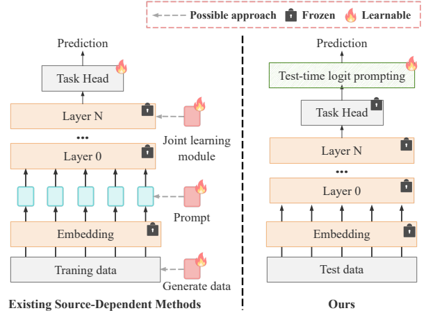
Figure 1: Comparison of the missing-modality adaptation paradigms. Existing source-dependent methods rely on training data for modality generation, prompt learning, or representation learning, whereas TLP adapts frozen VLMs at test time by optimizing lightweight logit prompts.
