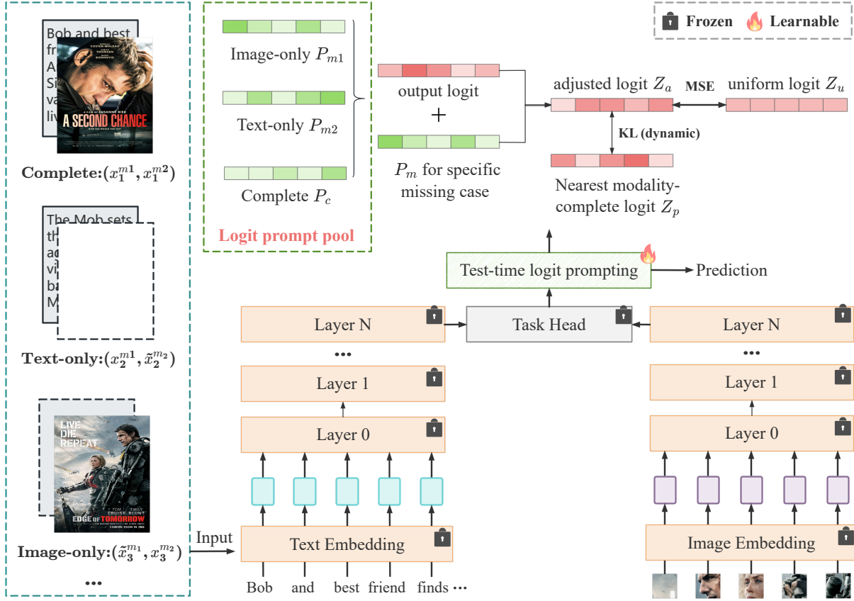
Figure 2: Overview of Test-Time Logit Prompting (TLP). Given a frozen VLM, TLP introduces missing-aware logit prompts to directly adapt the decision space under different missing-modality conditions. During inference, the corresponding logit prompt is selected according to modality availability and optimized through uncertainty-aware adjustment and modality-complete consistency regularization. The optimized prompt adjusts the original logits for final prediction, enabling efficient source-free missing-modality adaptation without updating the backbone.
