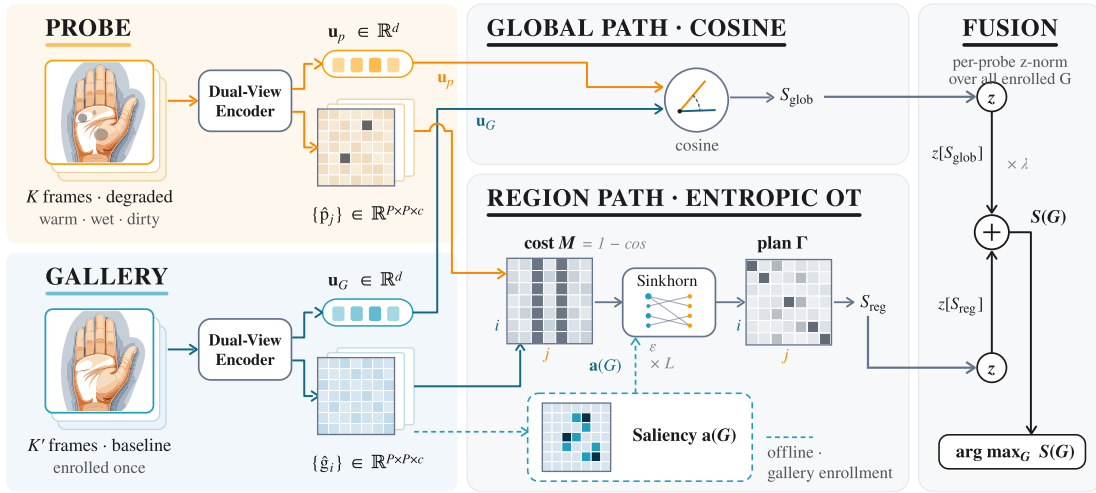
Fig. 5. Method Overview. A shared Dual-View Encoder (left) turns the probe clip and each enrolled gallery clip into a global embedding and a grid of regional features. From these, the test-time matcher scores a probe against each gallery: a region path (lower center) matched by entropic optimal transport, a global path (upper center) compared by cosine similarity, and a complementary fusion (right) that yields the final identity decision.
