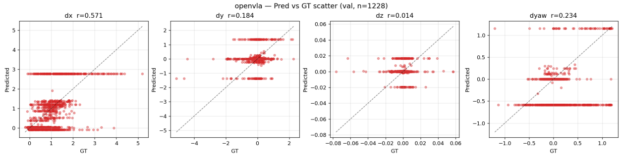
Figure D.3: Per-dimension prediction-vs.-ground-truth scatter for OpenVLA-7B on the held-out split. Note the horizontal banding caused by 256-bin discretization and the near-vertical collapse on \Delta z where the discretization grid resolution exceeds the empirical action range.
