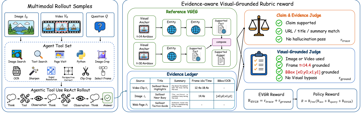
Figure 3 Overview of the Evidence-aware Visual-Grounded Rubric reward (EVGR). A task-level VEGG and evidence ledger align each multimodal rollout with the required visual anchors and source-supported facts. Claim-and-evidence and visual-grounding judges produce r_{\text{trace}} and r_{\text{ground}} , whose combination forms R_{\text{EVGR}} for policy optimization.
