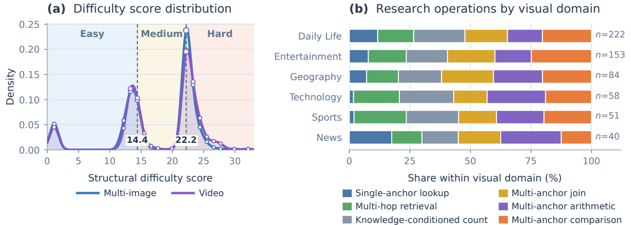
Figure 4 Benchmark distributions. (a) Smoothed structural-difficulty score distributions, with circles marking observed values. Dashed lines mark the empirical boundaries at 14.4 and 22.2; the easy, medium, and hard groups contain 100/100/101 multi-image and 102/102/103 video questions. (b) Operation composition within six visual domains. Bars are normalized within each domain, and n denotes the number of questions. Every domain covers all six principal research operations.
