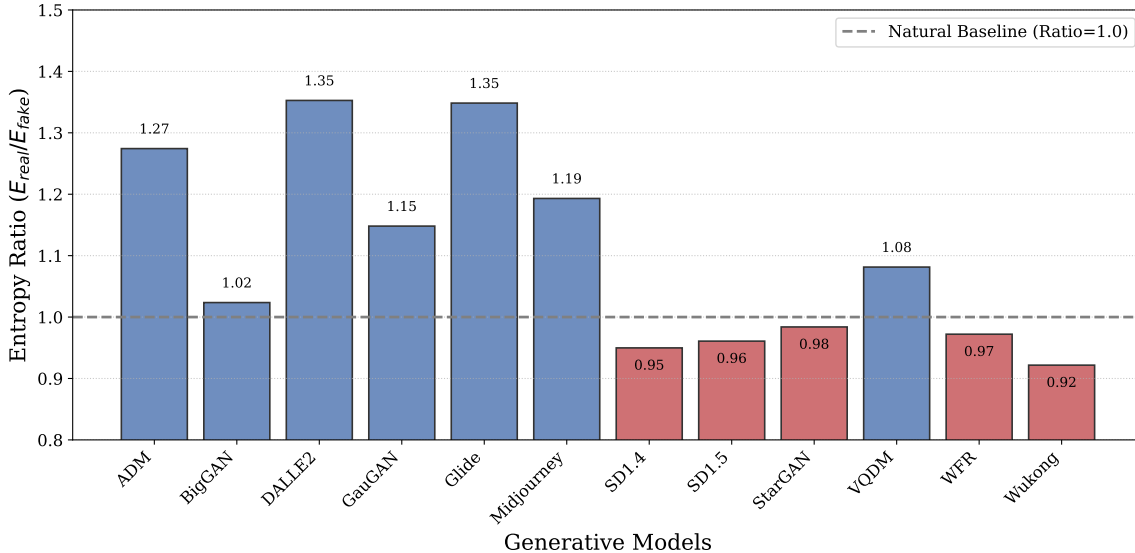
Figure 7: Exploratory GCM entropy ratios across 12 synthetic-image subsets. The dashed reference at one means equality of the two sample means, not equality of their full distributions. The original plot’s Natural Baseline label denotes this reference. Ratios both above and below one argue against a universal low-entropy detection rule.
