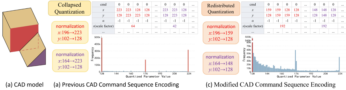
Figure 2: Revision of the DeepCAD parameter representation and its effect on parameter distributions: several parameters concentrate on very few valid values (e.g., most of x and y are concentrated at three specific values: 128, 176, and 223).
