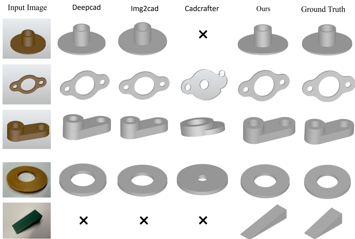
Figure 5: Qualitative comparison of image-to-CAD reconstruction results on synthetic and real-world image inputs. Our method produces more accurate geometric structures and dimensions compared with existing approaches, especially for complex objects under real-world conditions.
