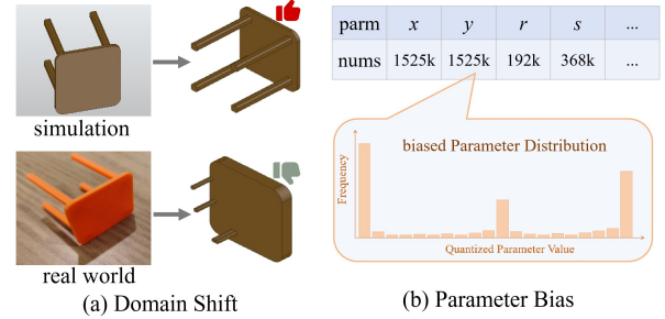
Figure 1: Key challenges in image-to-CAD reconstruction. (a) Domain shift : a model trained on synthetic renderings reconstructs synthetic inputs accurately but degrades substantially on real-world images (e.g., 3D printed CAD models). (b) Parameter bias : the DeepCAD representation produces highly concentrated geometric-parameter distributions, encouraging reliance on dataset-specific shortcuts.
