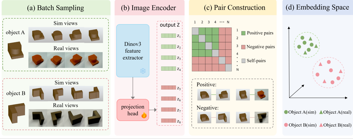
Figure 3: Overview of the feature-learning pipeline in RealCAD. Multi-view images from the synthetic and real domains are encoded by a frozen pretrained DINOv3 encoder and projected into a shared representation space, where multi-positive contrastive learning promotes cross-view and cross-domain consistency for the same CAD model.
