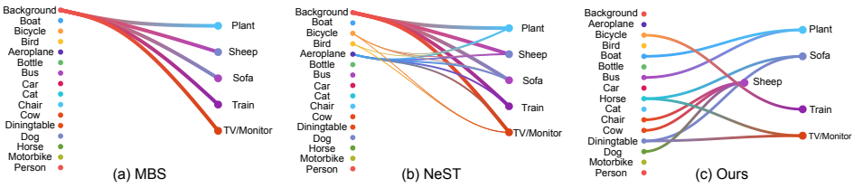
Figure 2: Visual representation of knowledge transfer in different approaches. (a) In MBS [65], the initial knowledge for incremental classes is transferred entirely from the background; (b) In NeST [49], most of the initial knowledge for incremental classes is transferred from the background; (c) In ours , the focus is on semantically relevant classes.
