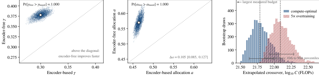
Figure 15: Conditional bootstrap uncertainty of the multimodal scaling fits and extrapolated crossover. Left: joint distribution of the encoder-free and encoder-based loss-compute exponents \gamma . Middle: joint distribution of their model allocation exponents a . Right: distributions of the extrapolated crossover compute under compute-optimal allocation and 5\times overtraining. Horizontal bars span the 10th to 90th percentiles, and dashed lines mark point estimates.
