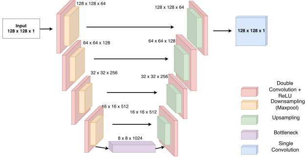
Figure 3. Modified U-Net Architecture. The encoder (left) consists of four double convolution blocks with ReLU activations, each followed by max pooling, progressively reducing the spatial dimensions from 128 \times 128 to 8 \times 8 while increasing the feature channels from 64 to 512. A bottleneck block at the deepest level expands the channels to 1024. The decoder (right) mirrors the encoder, restoring spatial resolution through upsampling and concatenating encoder feature maps via skip connections (horizontal arrows). A final 1 \times 1 convolution produces the output segmentation mask of size 128 \times 128 \times 1 .
