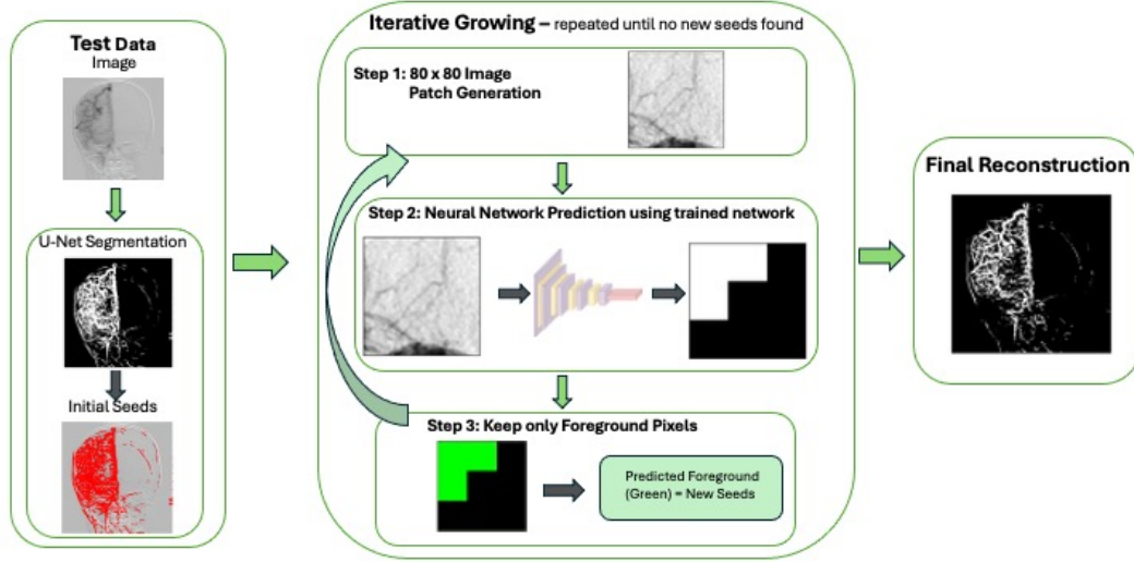
Figure 2. Proposed UI-VISA framework for vessel segmentation. The left panel shows a test image segmented by U-Net, with predicted foreground pixels (red) used as initial seeds. The middle panel illustrates the iterative seed expansion pipeline: 80 \times 80 image patches centered on current seeds are fed into a trained CNN to predict 3 \times 3 mask patches, with newly predicted foreground pixels added as seeds and the process repeated until convergence. The right panel shows the final reconstructed vessel segmentation.
