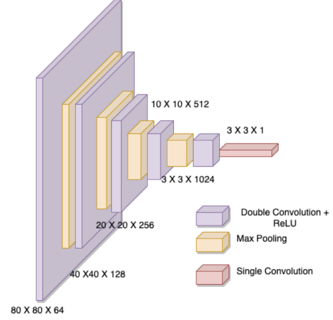
Figure 4. VISA Network Architecture: Convolutional neural network (CNN) architecture consisting of layers with double convolution and ReLU (purple), max pooling (yellow), and a final single convolution (red). The network takes an 80 \times 80 \times 1 grayscale patch as input. The dimensions labeled on each layer reflect the output of that layer, starting from 80 \times 80 \times 64 after the first double convolution and ending at 3 \times 3 \times 1 .
