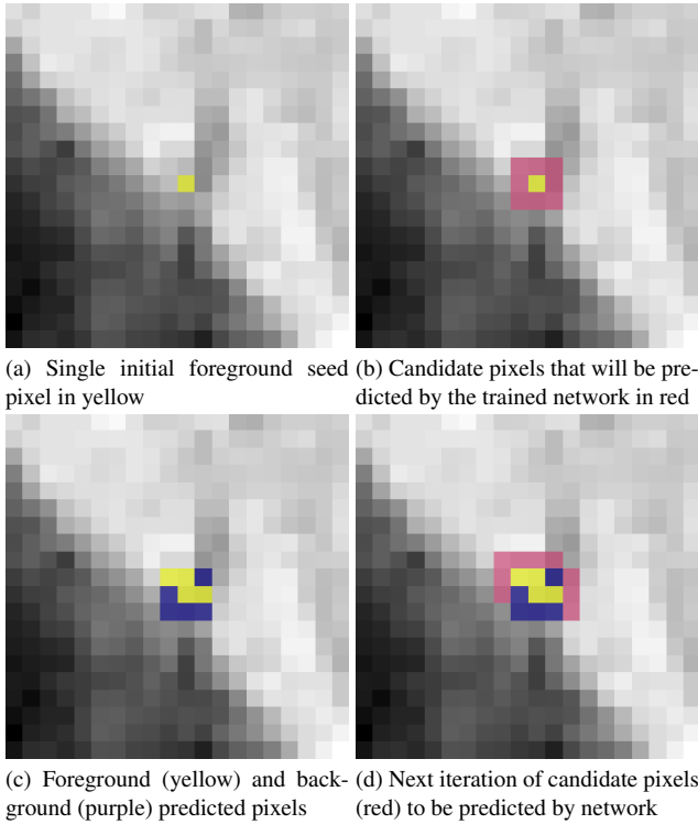
Figure 5. Illustration of Stage 2 of VISA. A single initial seed pixel (yellow) is shown in a. Panel b identifies the next candidate pixels (red) that will be evaluated by the trained network. Panel c shows the predicted classification of pixels into foreground (yellow) and background (purple). Panel d highlights the next set of candidate pixels (red) for the subsequent iteration of the network evaluation.
