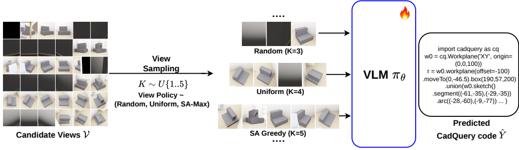
Figure 3: SightCAD generator warm-starting on variable- K multi-view subsets: candidate views are sampled under three view policies (random, uniform, SA-max) with K \sim \mathcal{U}\{1, \dots, 5\}
