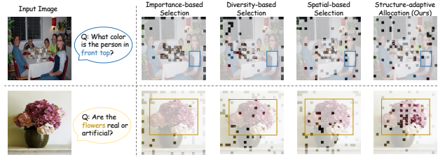
Figure 1. Comparison of four visual token selection strategies. Attention- and diversity-based methods exhibit spatial bias, while spatial-based selection preserves coverage but can miss important local details. S 2 Prune preserves broad coverage and allocates more tokens to structurally rich regions.
