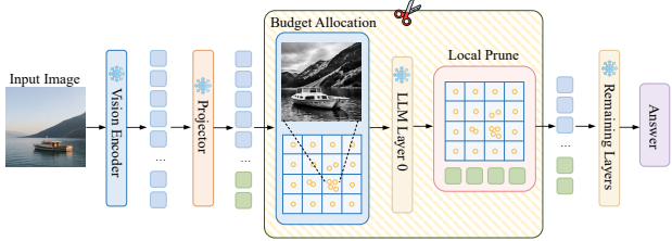
Figure 4. Overview of S^2 Prune. Regional image structure determines the spatial scaffold, after which early decoder responses select local representatives under the prescribed token budget.
