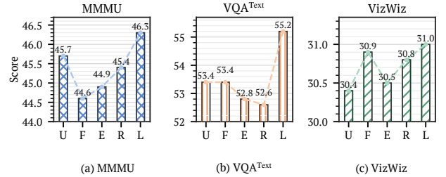
Figure 7. Structural-prior ablation at B = 64 . U/F/E/R/L denote Uniform, FFT, Effective Rank, Random, and Laplacian; Laplacian is best on all three tasks.
