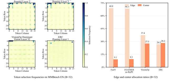
Figure S1. Spatial-bias measurements at B = 32 , extending Figures 2(b) and 2(c) of the main paper. The panel layout, 1,000 \text{MMB}^{\text{EN}} samples, score definitions, and pruning criteria are unchanged from the main-paper analysis; only the retained-token budget differs.
