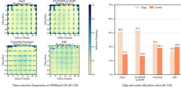
Figure S2. Spatial-bias measurements at B = 128 , extending Figures 2(b) and 2(c) of the main paper. The panel layout, 1,000 MMB EN samples, score definitions, and pruning criteria are unchanged from the main-paper analysis; only the retained-token budget differs.
