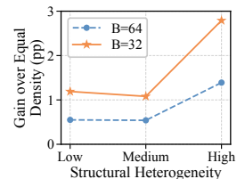
Figure 5. Gain of Adaptive over Equal Density on Qwen2.5-VL-7B, averaged over MMB^{EN} , VQA^{Text} , and POPE. Gains generally increase with structural heterogeneity, especially at B = 32 .
