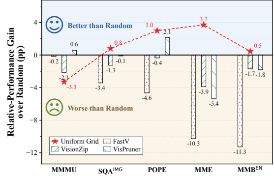
Figure 3. Performance-retention differences from Random on Qwen2.5-VL-7B at B = 64 . Values are percentage-point differences in retention relative to the unpruned 576-token model; zero denotes Random. Uniform Grid improves four of five benchmarks.
