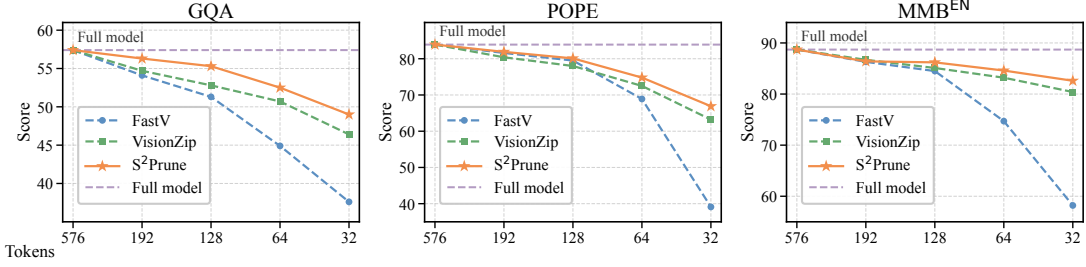
Figure 6. Qwen2.5-VL-7B performance across retained visual-token budgets on GQA, POPE, and \text{MMB}^{\text{EN}} . Dashed lines denote the unpruned 576-token model.
