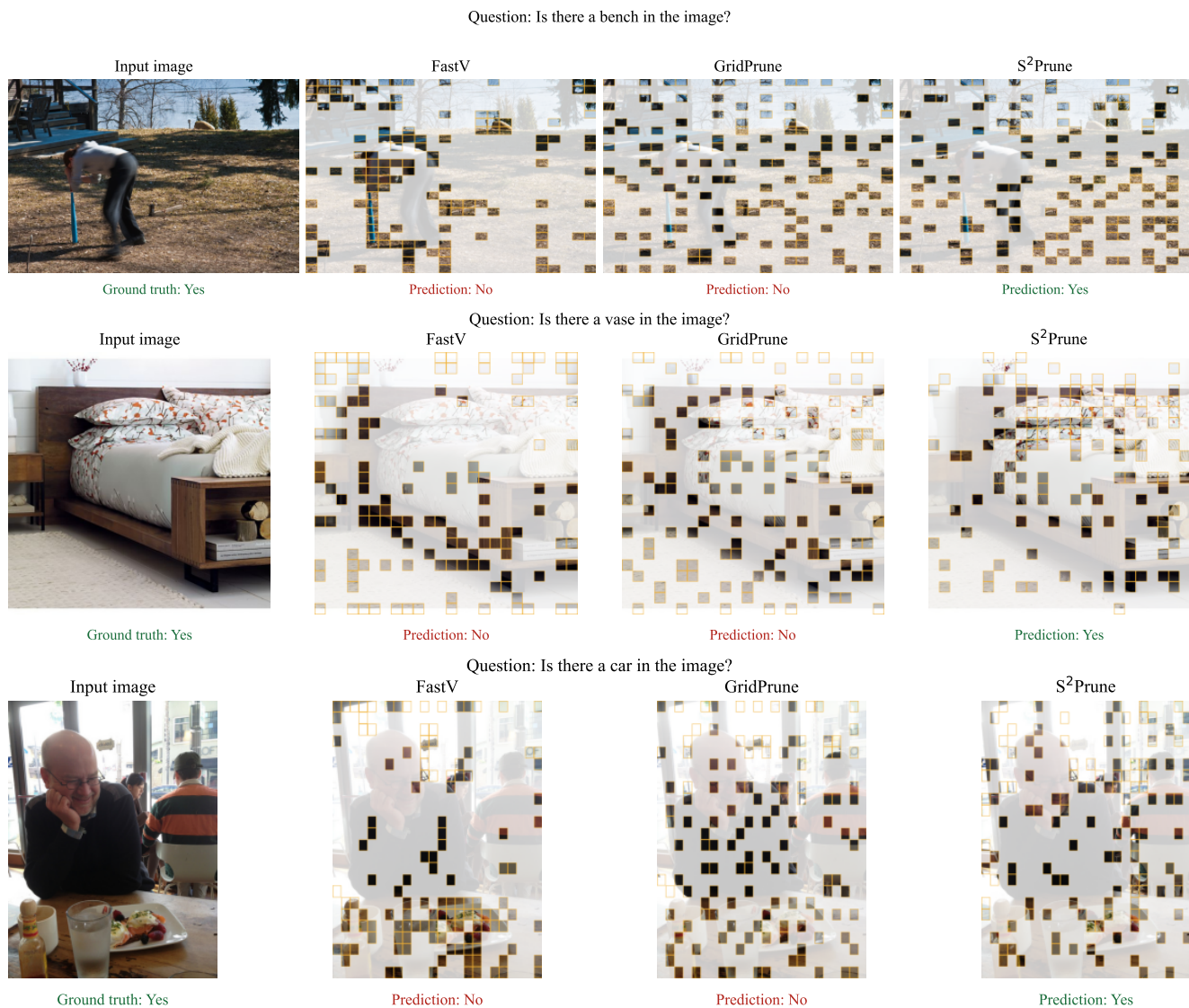
Figure S5. At B = 128/576 , S 2 Prune answers all three POPE queries correctly, whereas FastV and GridPrune answer incorrectly. The queries concern a bench, vase, and car; green and red text indicate correct and incorrect predictions, respectively.
