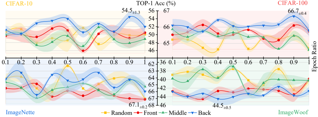
Figure 4: Hyperparameter study of SUA and ISS. On CIFAR-10/100 and ImageNette/Woof, we set \text{IPC} = 10 and use ResNet18 as both the teacher and student. We investigate the forward epoch ratio r_{\text{fwd}} \in \{0.1, 0.2, \dots, 1.0\} in SUA and the screening method (Random, Front, Middle, Back) in ISS.
