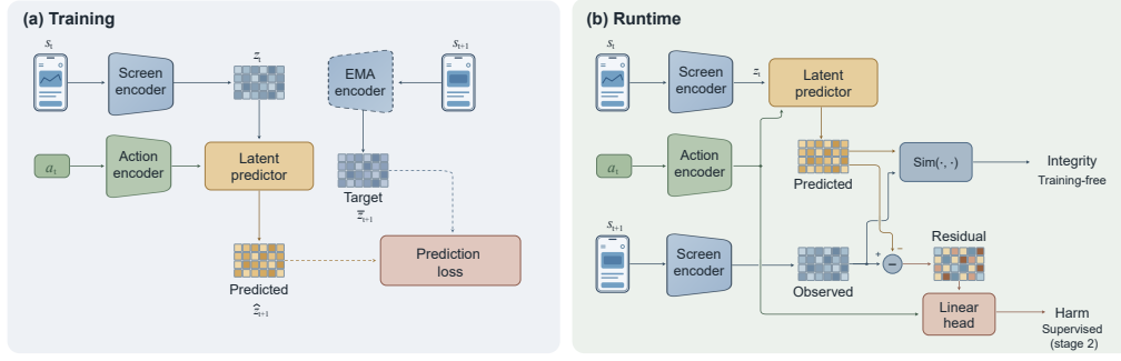
Figure 2: One predicted future, two closed-form readouts. (a) Training : an online screen encoder and spatially grounded action tokens condition a latent predictor; an EMA encoder supplies the next-state target, and changed patches receive higher loss weight. There is no decoder anywhere in the model. (b) Runtime : because predicted and observed futures share one space, the alignment gap gives a training-free integrity score (surprise detects), while the directional residual feeds a linear head that separates harmful from benign violations (direction interprets). Training-only paths are dashed.
