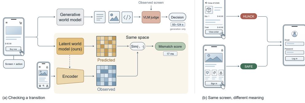
Figure 1: The future as an interface. (a): Existing GUI world models render the future as text, pixels, or code, at a cost of seconds to minutes per decision. LGWM predicts the future in representation space, in milliseconds. (b): A pixel-identical credential screen is legitimate after Sign in but hostile after View order . Safety is a property of the transition, not the screen.
