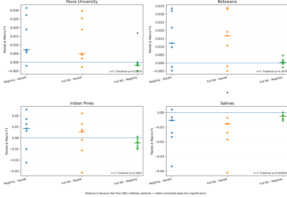
Figure 4: Paired dataset-level Macro-F1 changes under seven-fold stratified evaluation. Post-hoc testing is performed only when the dataset-level Friedman omnibus test is significant.
