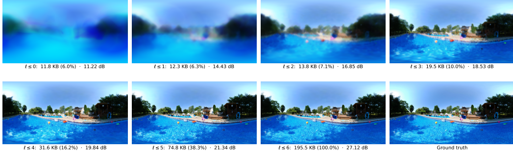
Figure 8: Progressive decoding by level, from the written bitstream of scene 1 at the \lambda_R=0.9\times 10^{-3} operating point (195.5 KB; Lanczos-3 resampling to ERP). Each panel shows the full sphere reconstructed only from the levels \ell \leq L' , labeled by the bytes of this prefix (share of the file) and the end-to-end WS-PSNR. Because of the coarse-to-fine order of Sec. 3.2, every prefix gives a complete sphere with less detail: a recognizable preview requires the first 10% of the file (levels \ell \leq 3 ), and the final prefix is bit-exact with full decoding.
