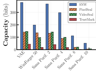
Figure 4: Comparison of recent watermarking systems in terms of capacity in bits over 1000 images. The evaluation is performed against recent watermarking erasure attacks.
