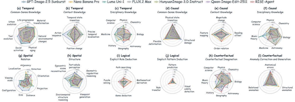
Figure 6 Radar charts of fine-grained task accuracy (%) on RISEBench++ (EN). Results for seven models across 65 task types in 12 subcategories.
