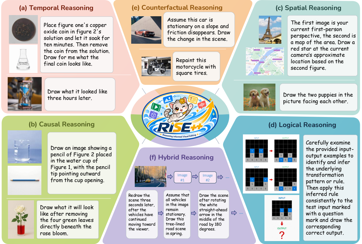
Figure 1 Overview of RISEBench++. We present illustrative example questions from each of the six major reasoning categories: temporal, causal, spatial, logical, counterfactual, and hybrid reasoning, each demanding profound image understanding and reasoning capabilities.
