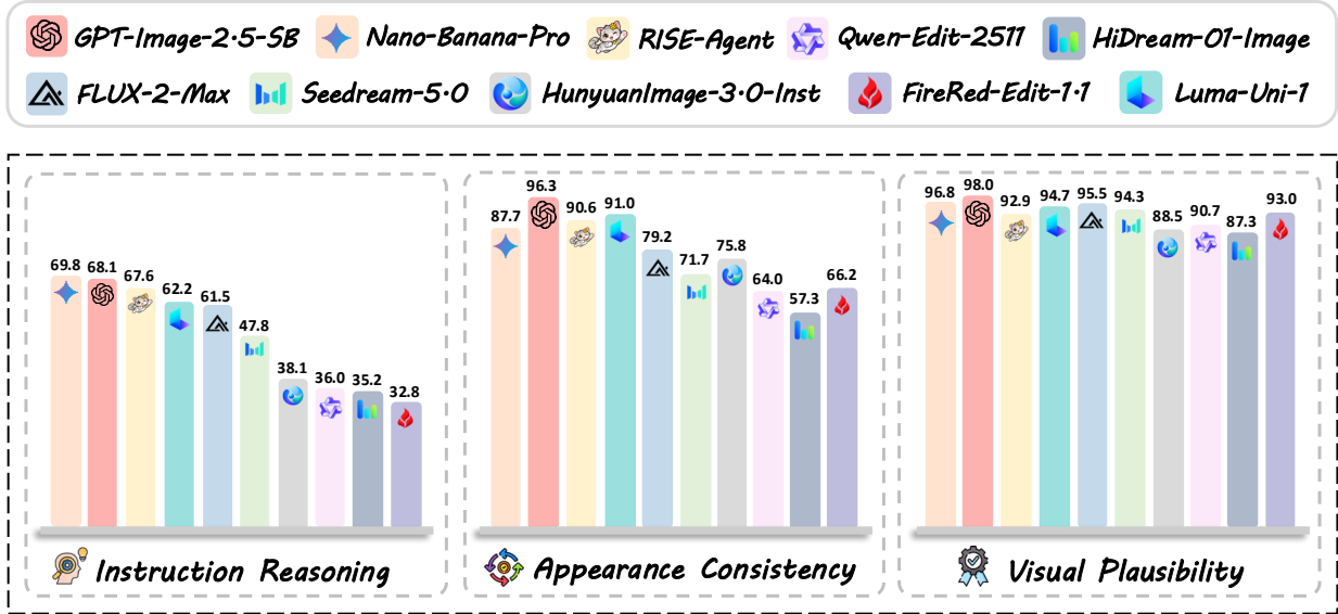
Figure 5 Comparison across three evaluation dimensions on RISEBench++ (EN). Nano Banana Pro achieves the highest instruction reasoning score, while GPT-Image-2.5 Sunburst leads in appearance consistency and visual plausibility.
