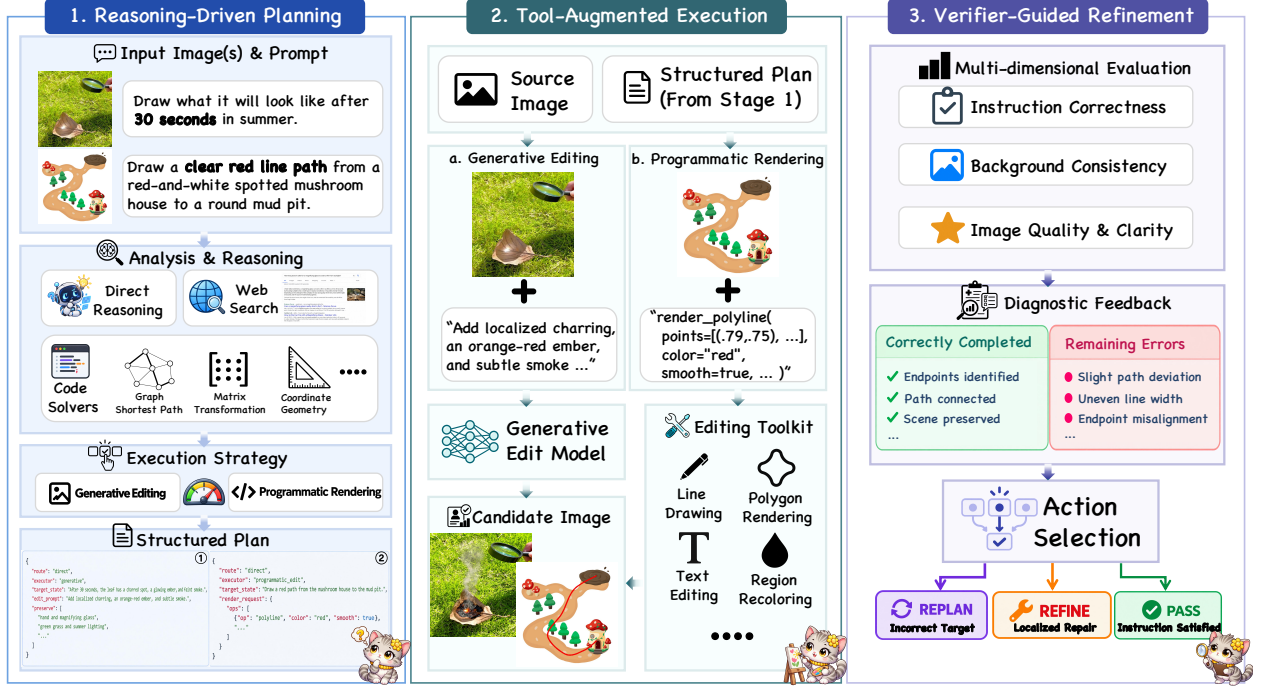
Figure 4 Overview of RISE-Agent. RISE-Agent follows a closed-loop workflow of reasoning-driven planning, tool-augmented execution, and verifier-guided refinement, bridging target-state inference with precise visual realization.
