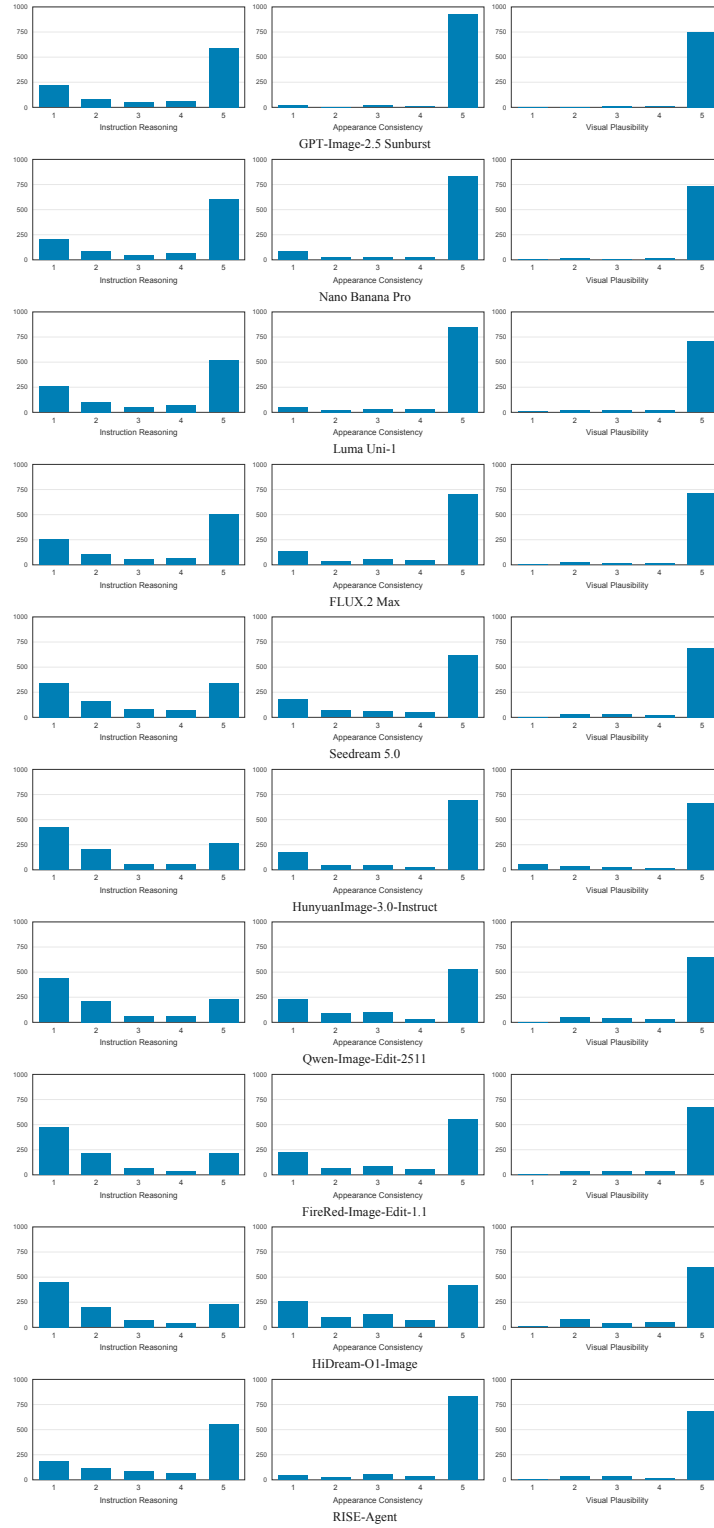
Figure 8 Score distributions on RISEBench++ (EN). Results for ten models across 1,000 cases. The three columns report Instruction Reasoning (IR), Appearance Consistency (AC), and Visual Plausibility (VP). Bars count cases at each score from 1 to 5.
