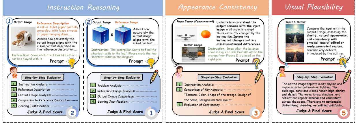
Figure 3 Evaluation metrics and pipeline of RISEBench++. RISEBench++ evaluates generated images across Instruction Reasoning , Appearance Consistency , and Visual Plausibility . Gemini-3-Flash evaluates the first two using dimension-specific prompts, while Gemini-3.1-Flash-Lite evaluates the third.
