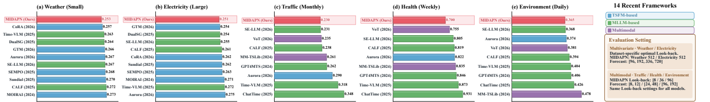
Fig. 6. TFSMs, fused-PLMs and multimodal frameworks comparison (sorted by averaged MAE from low to high). MIDAPN consistently achieves the lowest MAE across the selected benchmarks, highlighting its accuracy advantage over pretrained forecasting approaches under extended look-back settings
